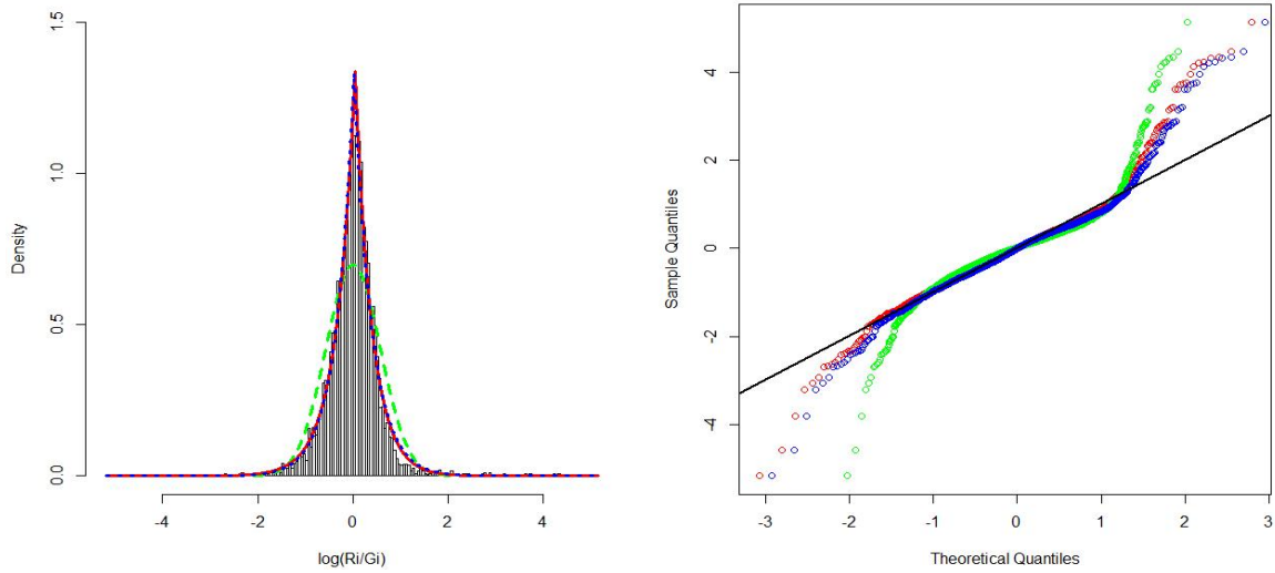
Fig. 13. Left panel: Histogram of Ecoli.4 superimposed with Esscher transformed Laplace (red line), Laplace (blue dotted) and Normal (green dashed) distributions. Right panel: Q-Q plot of Esscher transformed Laplace (red), Laplace (blue) and Normal (green) distributions.
