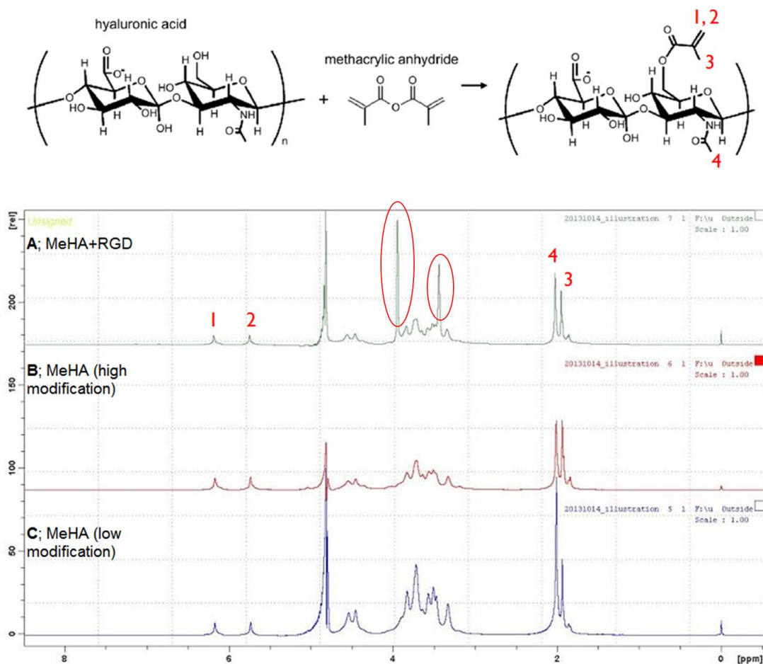
Figure A-2. NMR spectra
