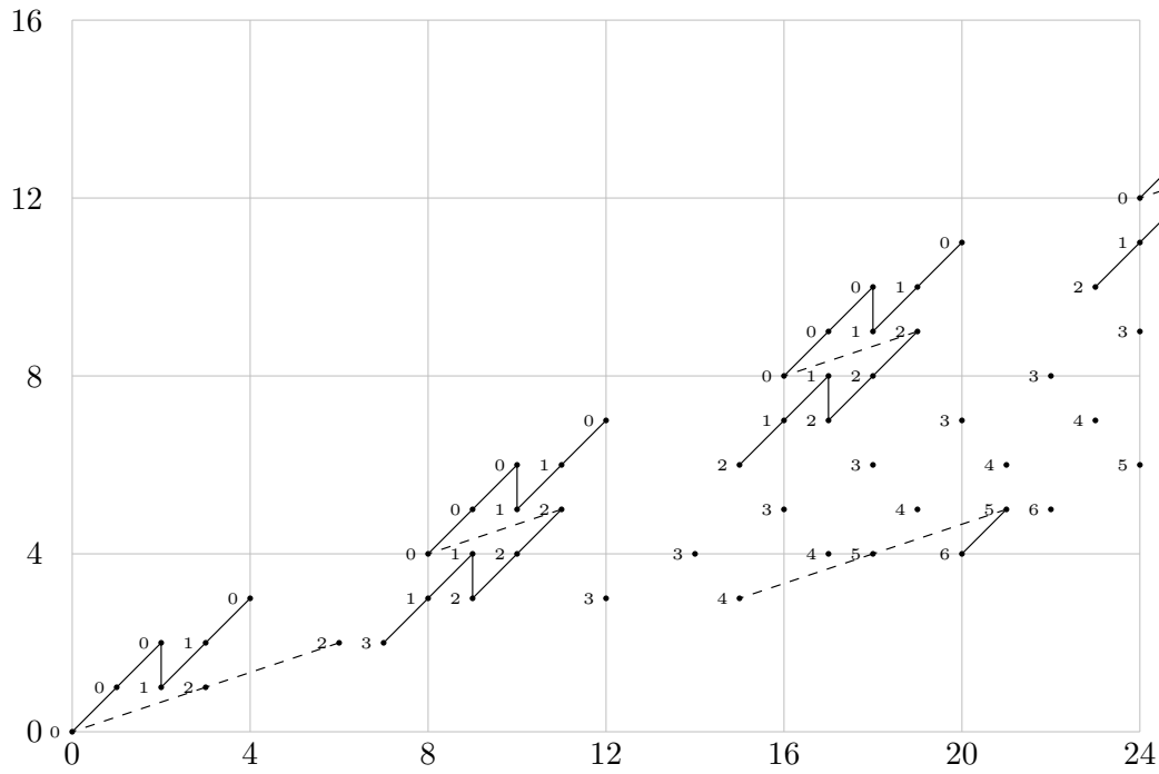
FIGURE 1.24. \text{Ext}_{A(2)}^{s,t}(M_1, \mathbb{F}_2) for 0 \leq t - s \leq 24
