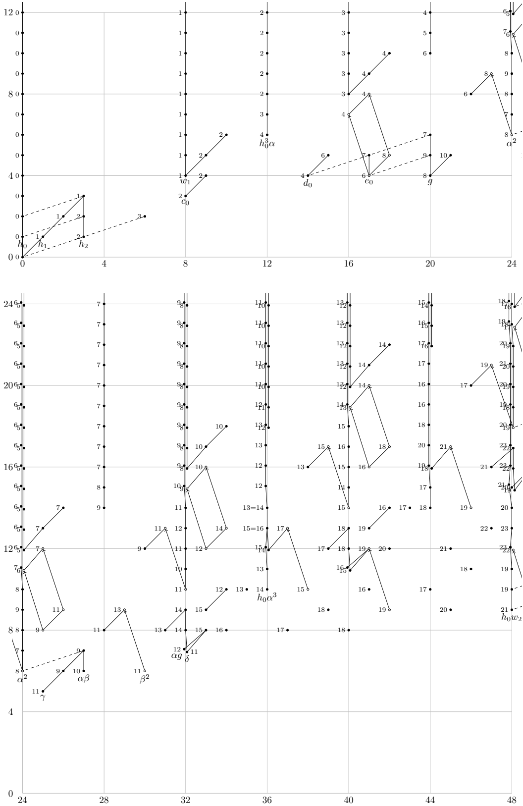
FIGURE 0.2. (E_3(tmf), d_3) for t - s \leq 48
