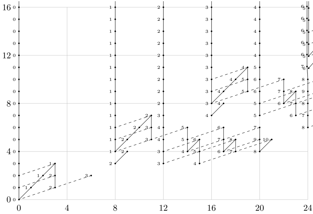
FIGURE 1.11. \text{Ext}_{A(2)}^{s,t}(\mathbb{F}_2, \mathbb{F}_2) for 0 \leq t - s \leq 24
