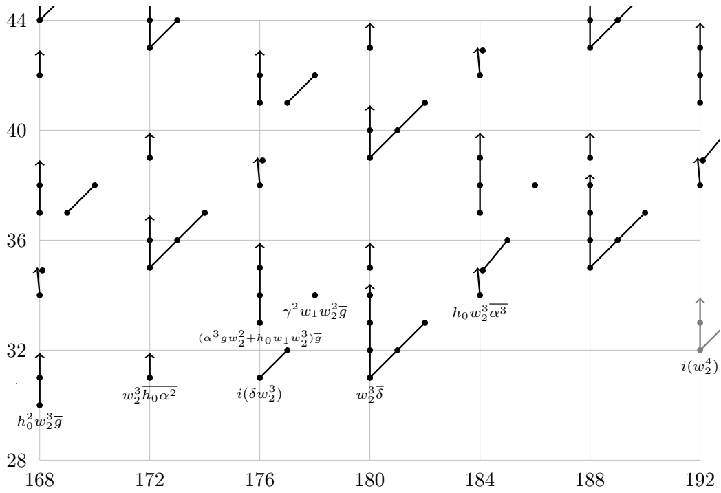
FIGURE 8.8. E_5(tm\mathbf{f}/\nu) = E_\infty(tm\mathbf{f}/\nu) for 168 \leq t - s \leq 192
