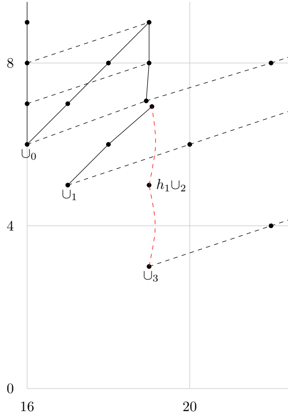
FIGURE 11.6. Delayed E_\infty -term for \pi_*(\Sigma^8 P_8^\infty)
