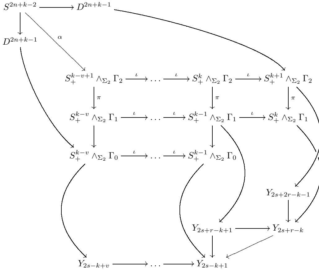
FIGURE 11.3. Maps from two hemispheres
