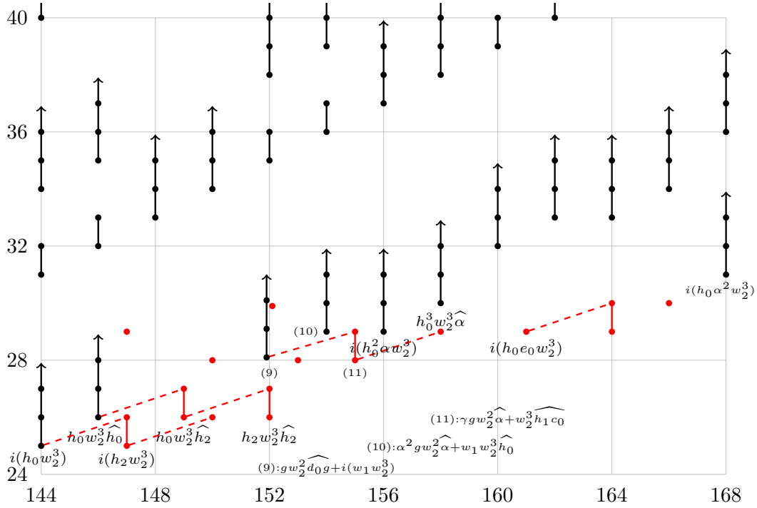
FIGURE 7.7. E_4(tm\mathbf{f}/\eta) = E_\infty(tm\mathbf{f}/\eta) for 144 \leq t - s \leq 168
