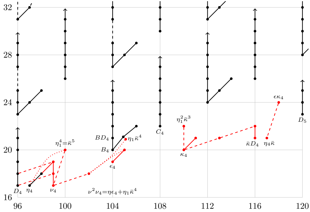
FIGURE 9.10. \pi_n(tmf) for 96 \leq n \leq 120
