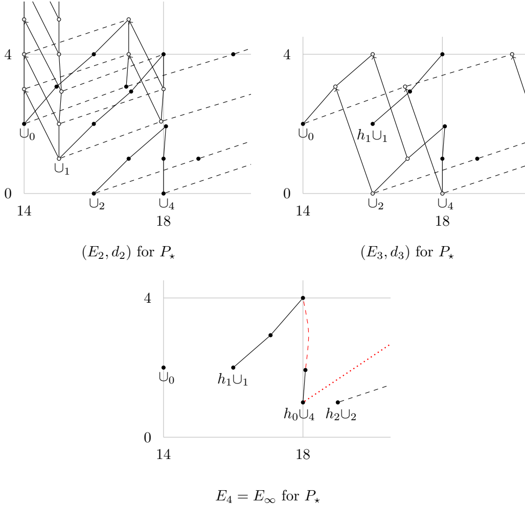
FIGURE 11.4. Delayed Adams spectral sequence for \pi_*(\Sigma^7 P_7^\infty)
