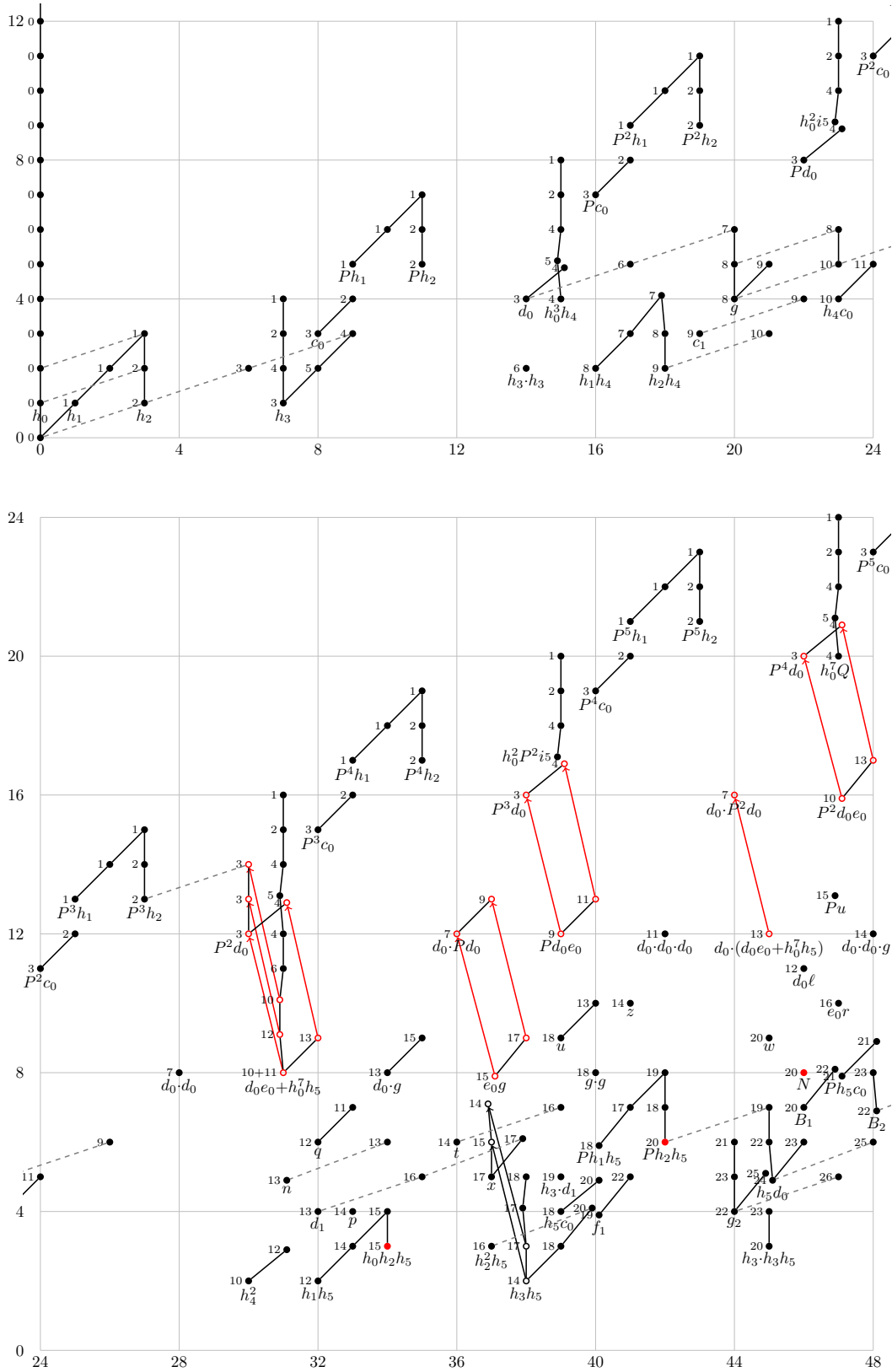
FIGURE 11.12. (E_4(S), d_4) for t - s \leq 48
