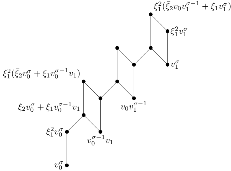
FIGURE 3.2. The syzygy \Omega_{A(1)_*}^\sigma(E(\xi_1^2)) for \sigma = 3
