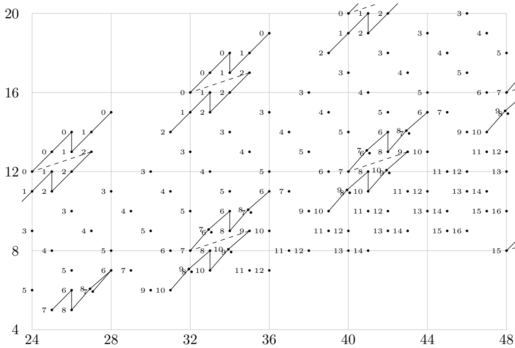
FIGURE 1.25. \text{Ext}_{A(2)}^{s,t}(M_1, \mathbb{F}_2) for 24 \leq t - s \leq 48
