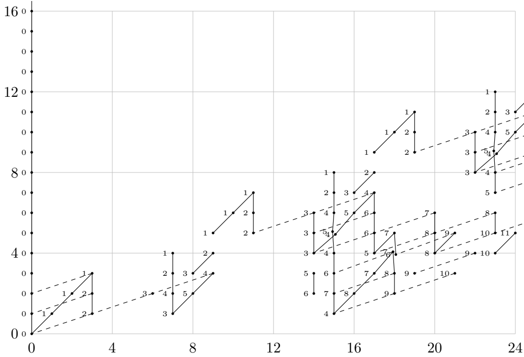
FIGURE 1.1. \text{Ext}_A^{s,t}(\mathbb{F}_2, \mathbb{F}_2) for 0 \leq t - s \leq 24
