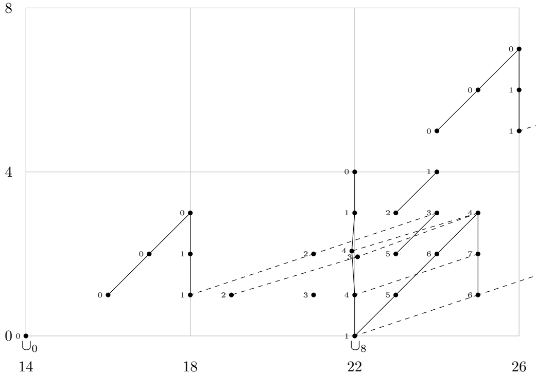
FIGURE 11.5. Adams spectral sequence for \pi_*(\Sigma^7 P_7^\infty)
