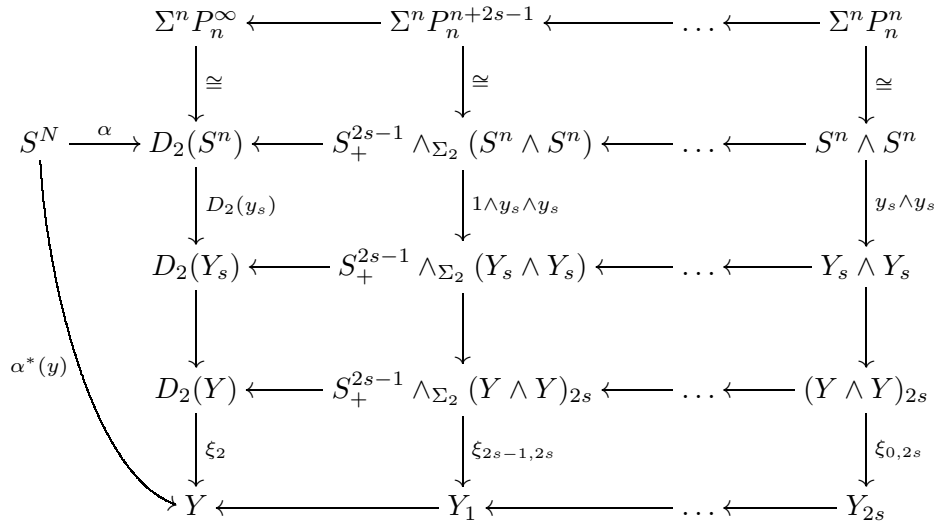
FIGURE 11.1. Factorization of power operation \alpha^*(y)
