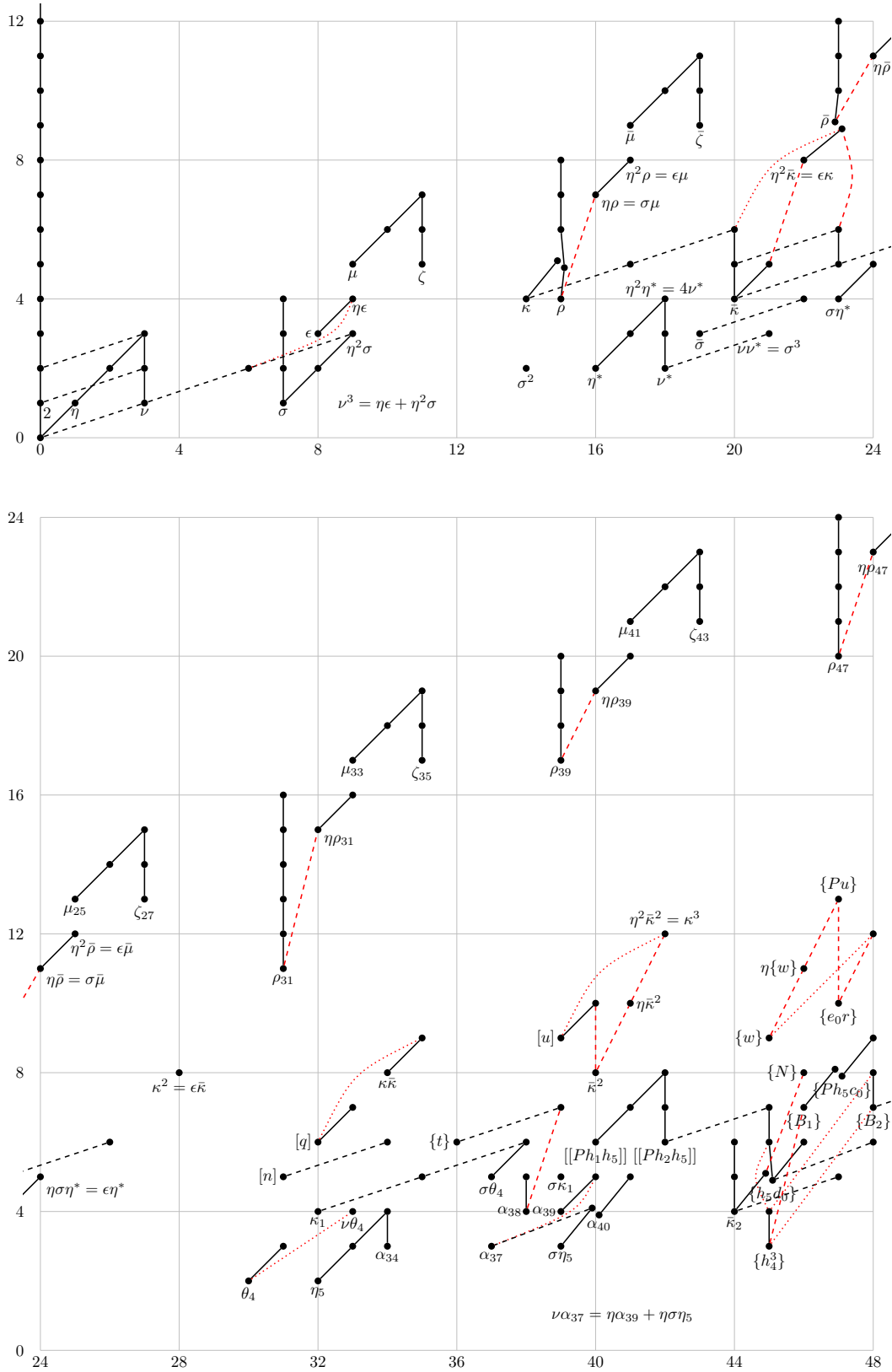
FIGURE 11.14. \pi_n(S) for n \leq 48
