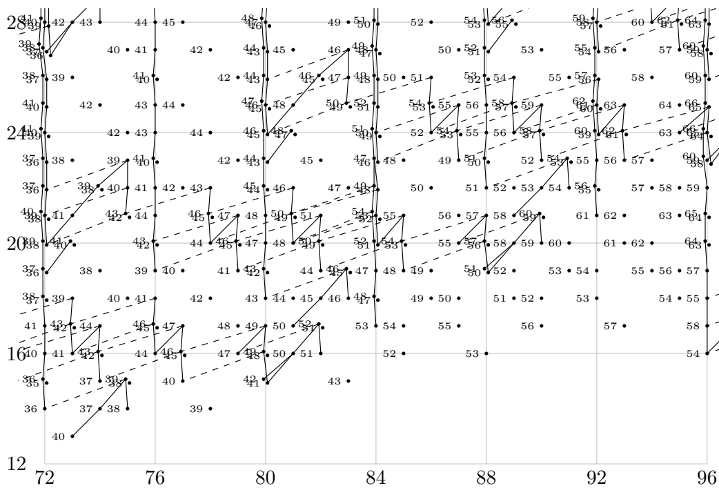
FIGURE 1.14. \text{Ext}_{A(2)}^{s,t}(\mathbb{F}_2, \mathbb{F}_2) for 72 \leq t - s \leq 96
