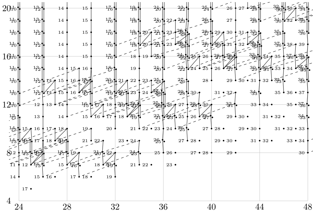
FIGURE 1.29. \text{Ext}_{A(2)}^{s,t}(M_2, \mathbb{F}_2) for 24 \leq t - s \leq 48
