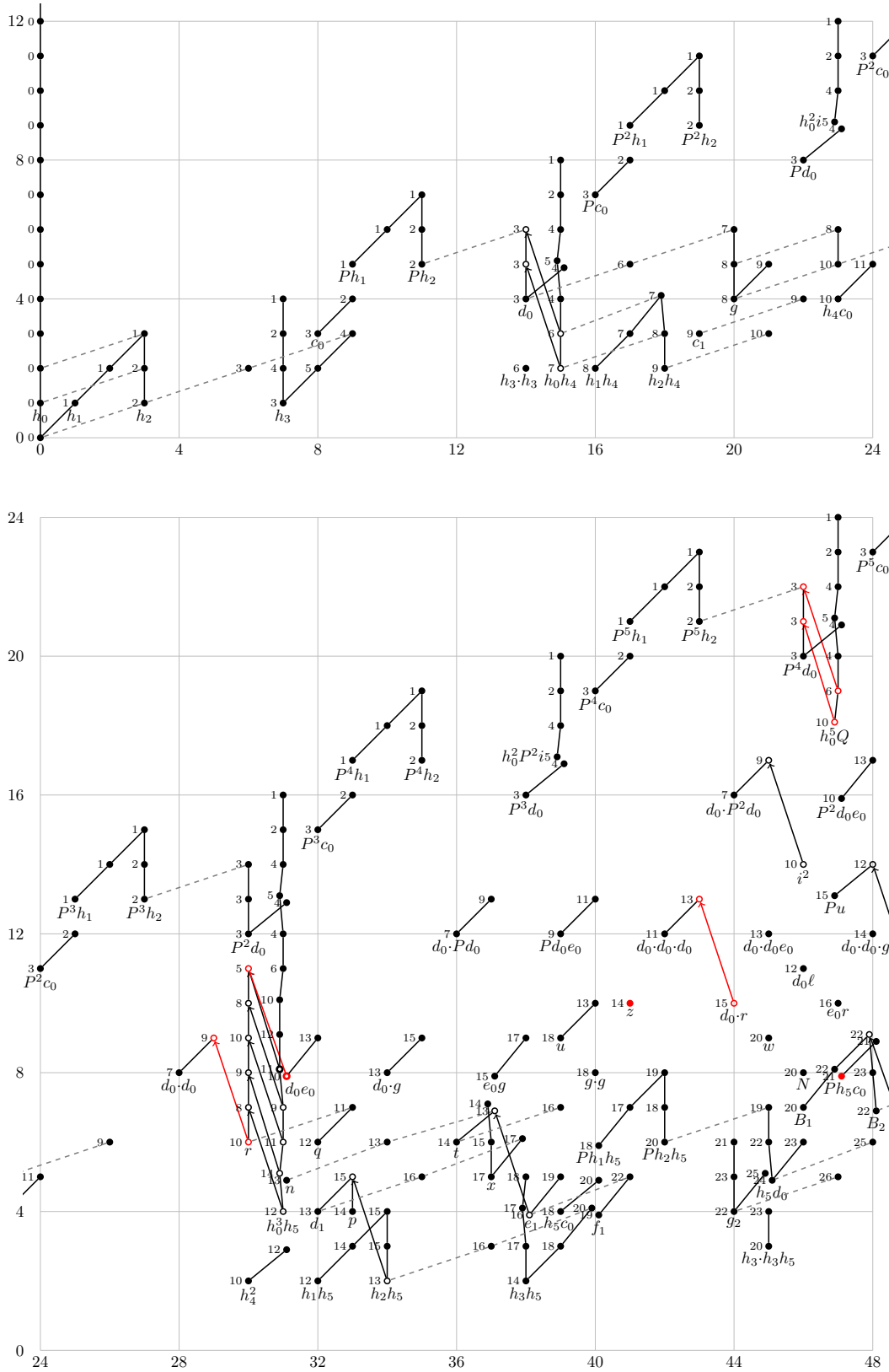
FIGURE 11.11. (E_3(S), d_3) for t - s \leq 48
