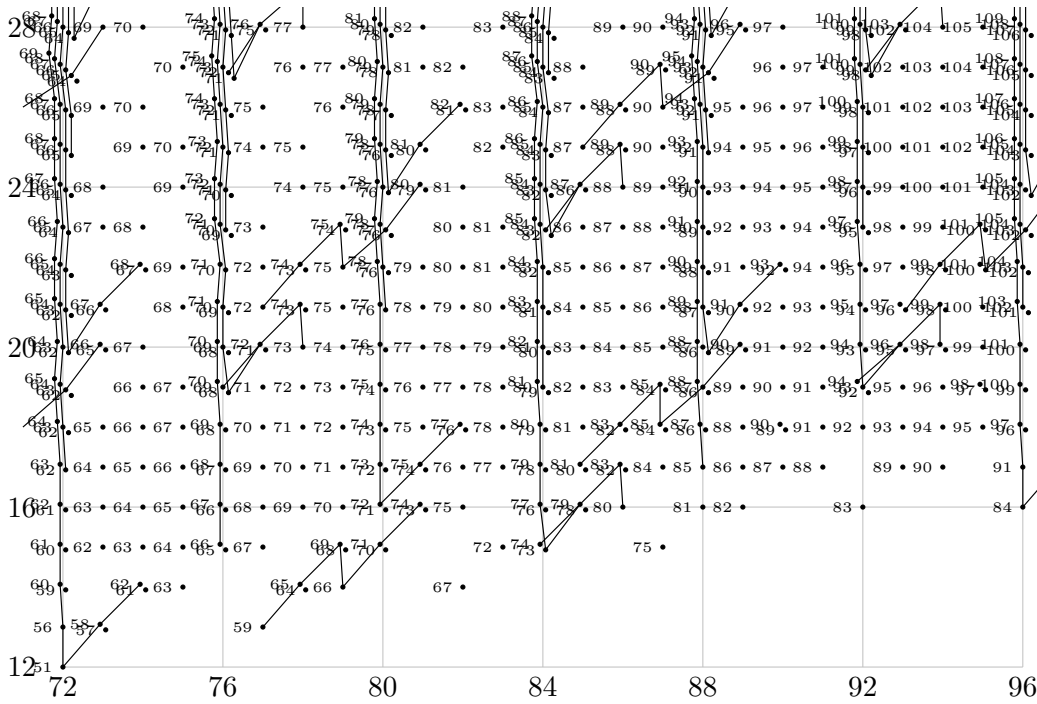
FIGURE 1.35. \text{Ext}_{A(2)}^{s,t}(M_4, \mathbb{F}_2) for 72 \leq t - s \leq 96
