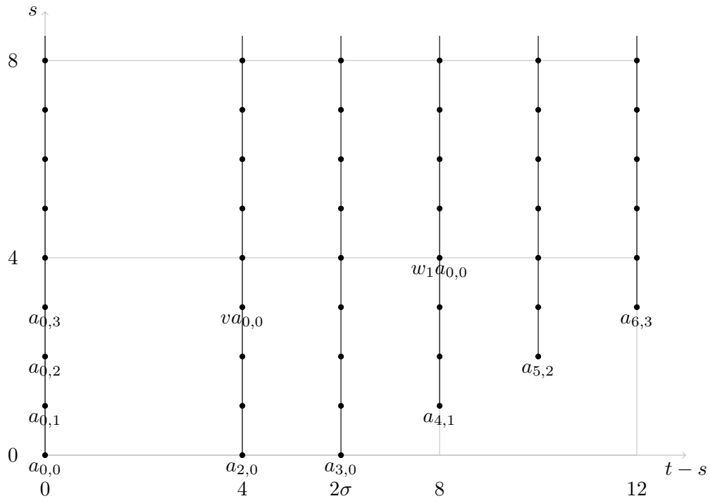
FIGURE 3.6. The Adams chart G\langle\sigma\rangle^{*,*} for \sigma = 3
