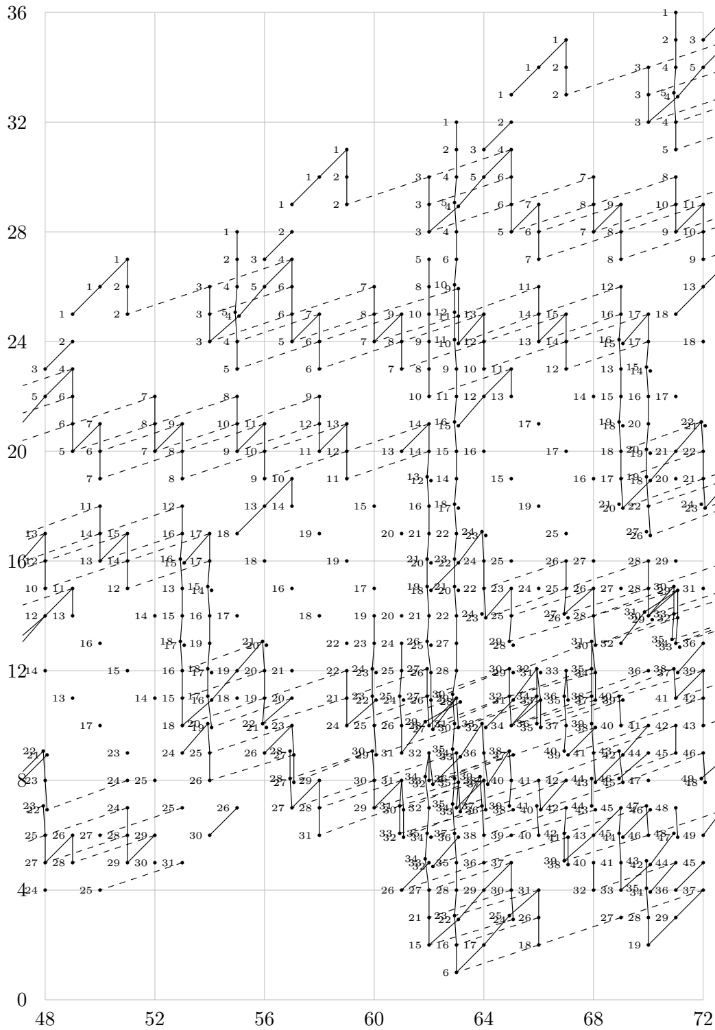
FIGURE 1.3. \text{Ext}_A^{s,t}(\mathbb{F}_2, \mathbb{F}_2) for 48 \leq t - s \leq 72
