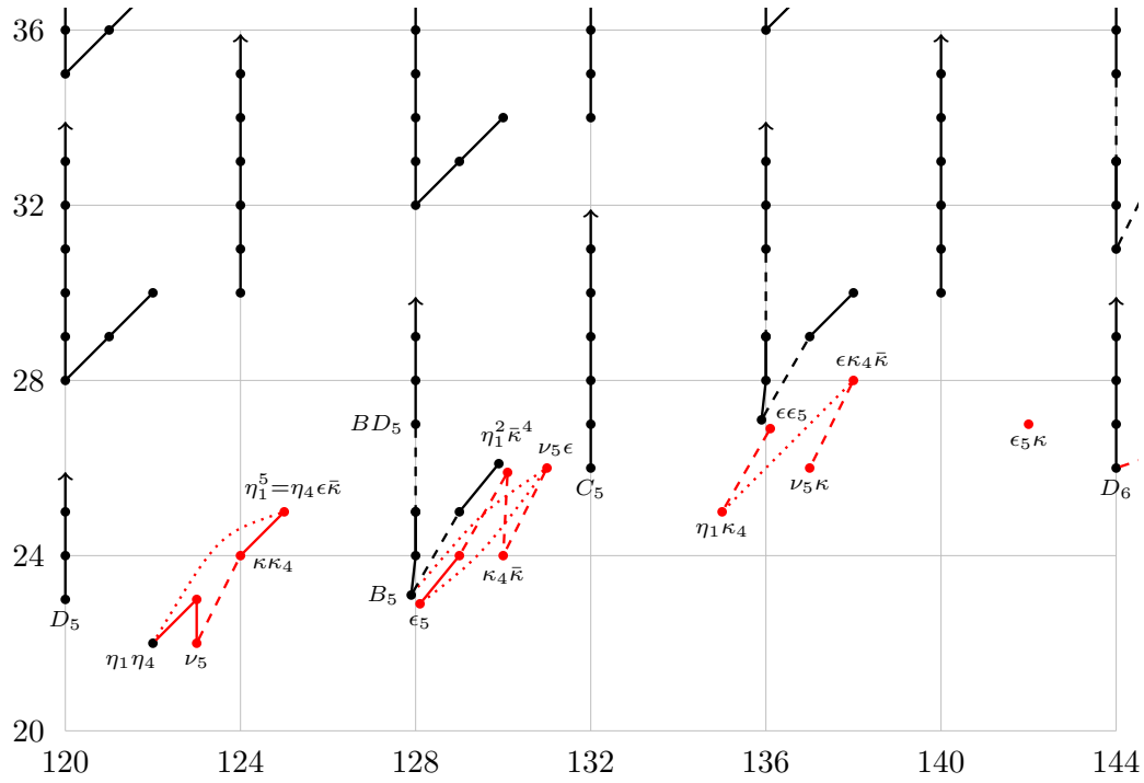
FIGURE 9.11. \pi_n(tmf) for 120 \leq n \leq 144
