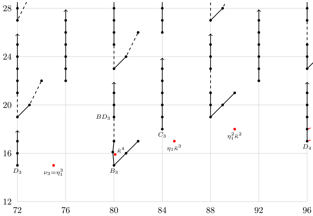
FIGURE 9.9. \pi_n(tmf) for 72 \leq n \leq 96
