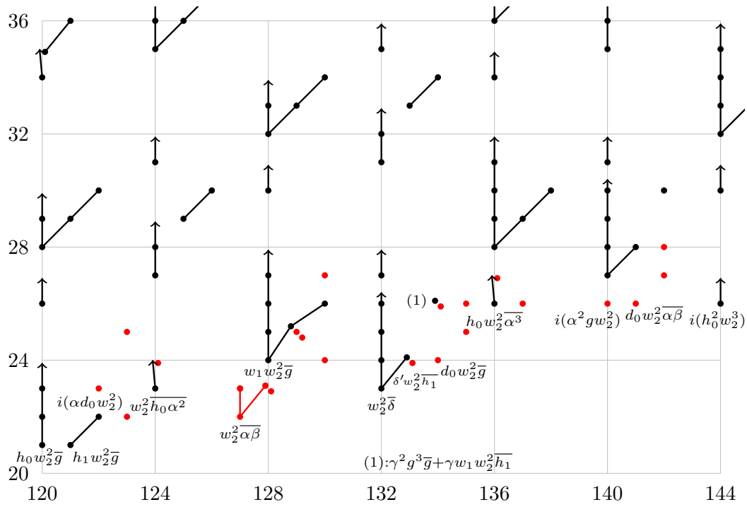
FIGURE 8.6. E_5(tm\mathbb{f}/\nu) = E_\infty(tm\mathbb{f}/\nu) for 120 \leq t - s \leq 144
