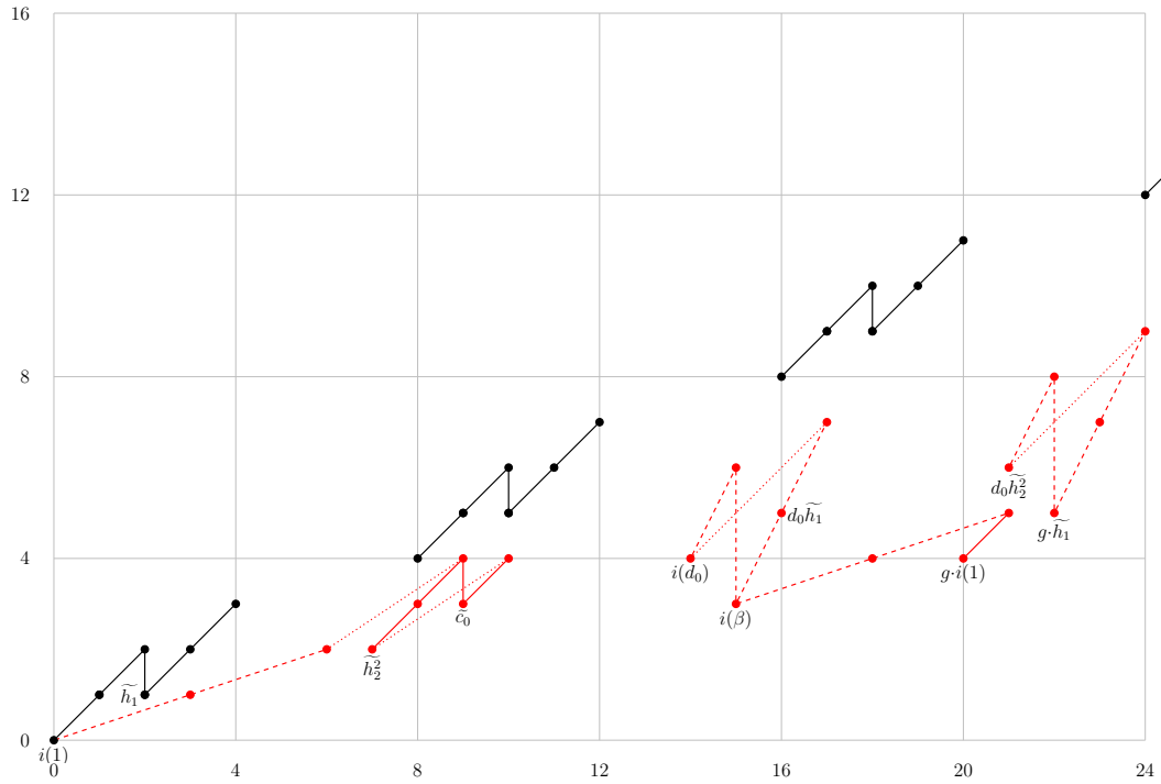
FIGURE 12.1. E_\infty(tm\!f/2) for 0 \leq t - s \leq 24 , with all hidden 2-, \eta - and \nu -extensions
