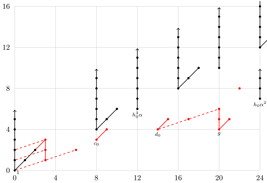
FIGURE 5.1. E_5(tm_f) = E_\infty(tm_f) for 0 \leq t - s \leq 24
