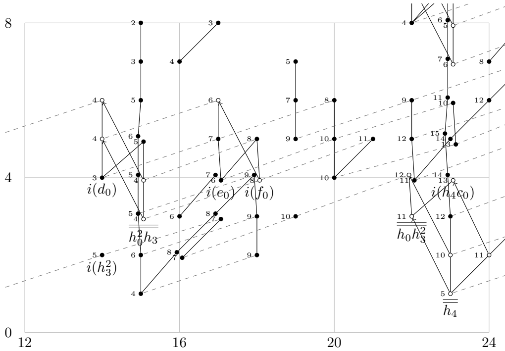
FIGURE 11.15. (E_2(C\sigma), d_2) for 12 \leq t - s \leq 24
