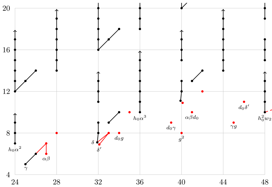
FIGURE 5.2. E_5(tm_f) = E_\infty(tm_f) for 24 \leq t - s \leq 48
