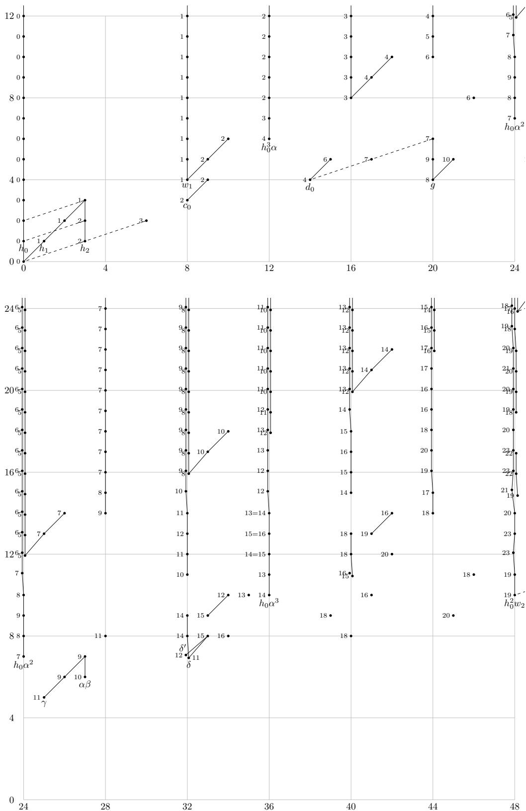
FIGURE 0.4. E_5(tmf) = E_\infty(tmf) for t - s \leq 48
