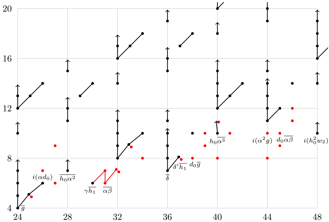
FIGURE 8.2. E_5(tm\mathbb{f}/\nu) = E_\infty(tm\mathbb{f}/\nu) for 24 \leq t - s \leq 48
