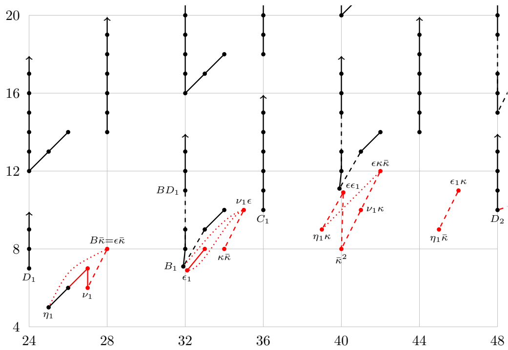
FIGURE 9.7. \pi_n(tmf) for 24 \leq n \leq 48
