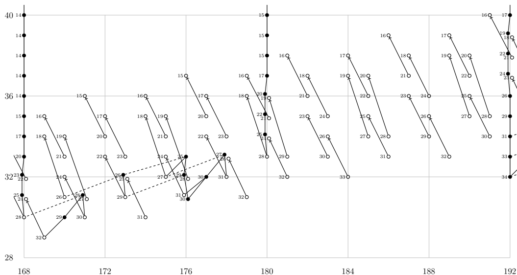
FIGURE 12.48. Hastened (E_r(tmf/B), d_r) for 168 \leq t - s \leq 192
