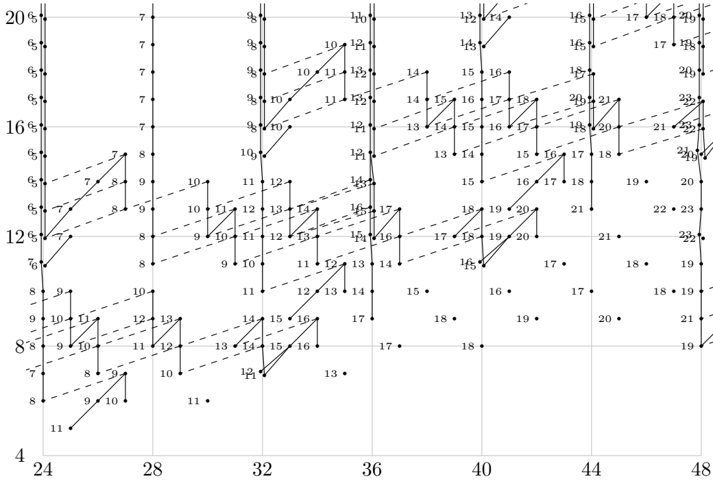
FIGURE 1.12. \text{Ext}_{A(2)}^{s,t}(\mathbb{F}_2, \mathbb{F}_2) for 24 \leq t - s \leq 48
