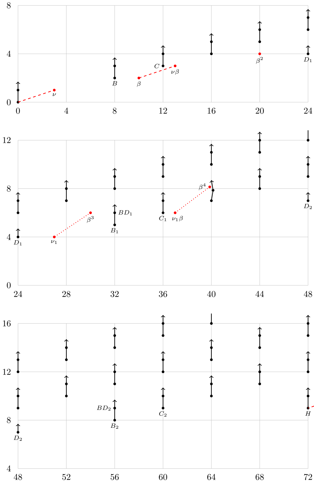
FIGURE 13.2. \pi_n(tmf) at p = 3 for 0 \leq n \leq 72
