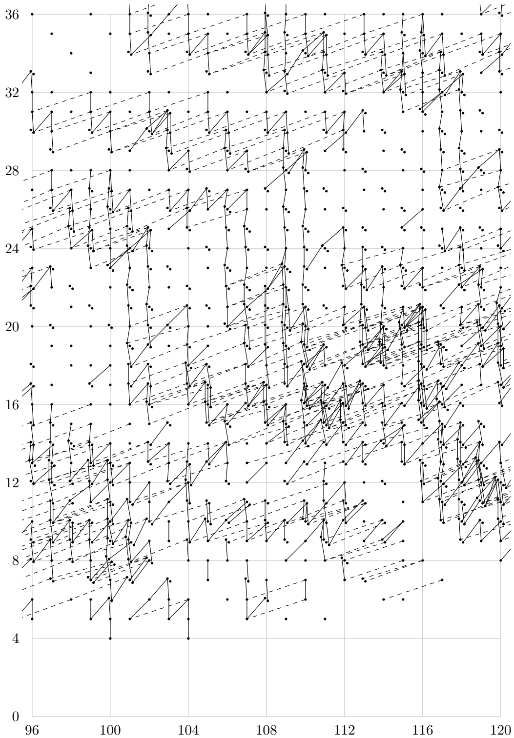
FIGURE 1.5. \text{Ext}_A^{s,t}(\mathbb{F}_2, \mathbb{F}_2) for 96 \leq t - s \leq 120
