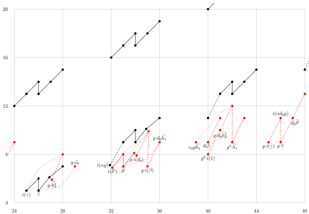
FIGURE 12.2. E_\infty(tm\!f/2) for 24 \leq t - s \leq 48 , with all hidden 2-, \eta - and \nu -extensions
