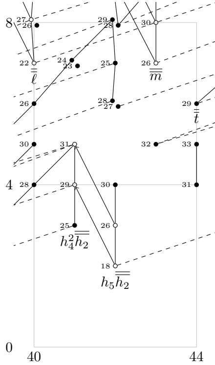
FIGURE 11.21. (E_2(C\sigma), d_2) for 40 \leq t - s \leq 44
