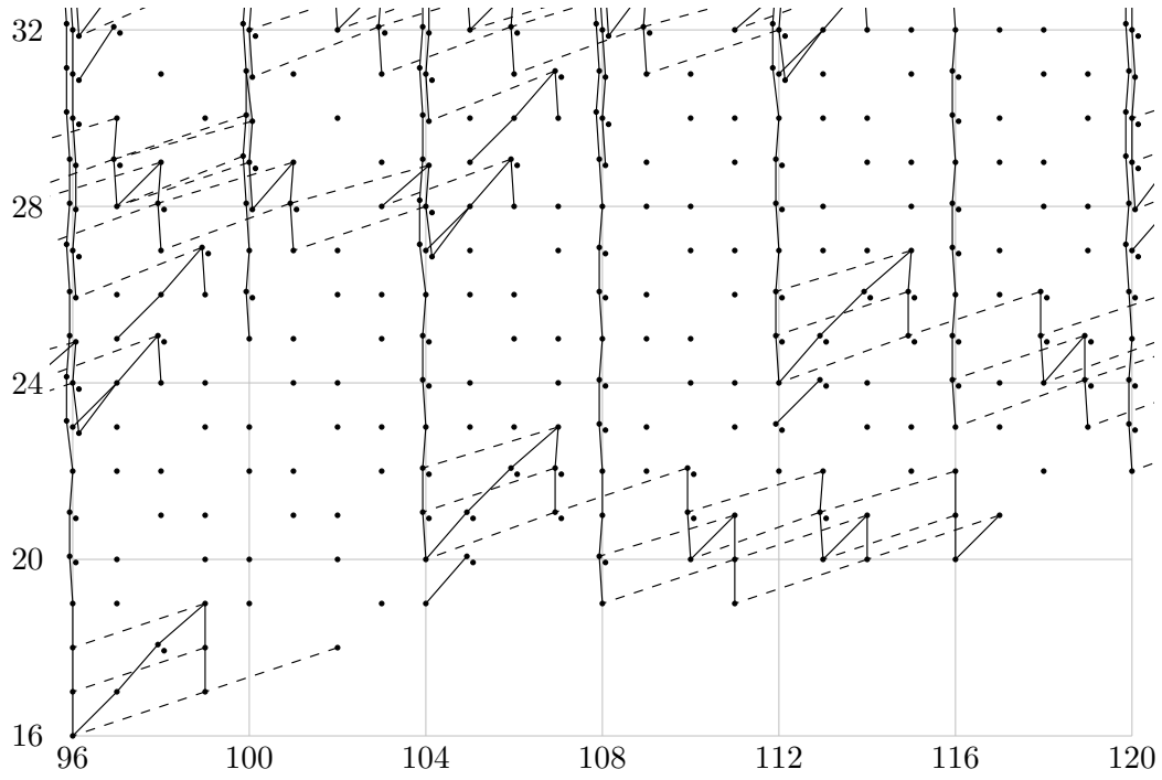
FIGURE 1.15. \text{Ext}_{A(2)}^{s,t}(\mathbb{F}_2, \mathbb{F}_2) for 96 \leq t - s \leq 120
