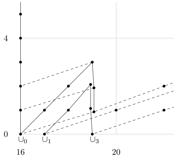
FIGURE 11.6. Delayed E_\infty -term for \pi_*(\Sigma^8 P_8^\infty)
