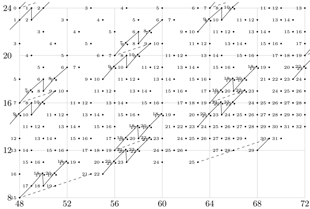
FIGURE 1.26. \text{Ext}_{A(2)}^{s,t}(M_1, \mathbb{F}_2) for 48 \leq t - s \leq 72
