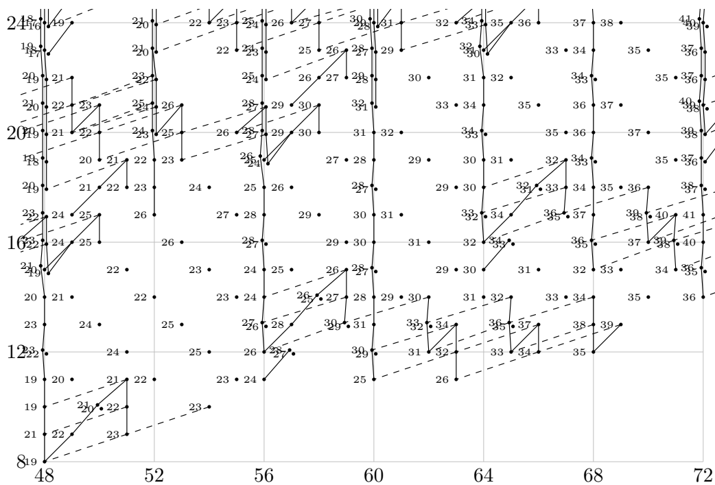
FIGURE 1.13. \text{Ext}_{A(2)}^{s,t}(\mathbb{F}_2, \mathbb{F}_2) for 48 \leq t - s \leq 72
