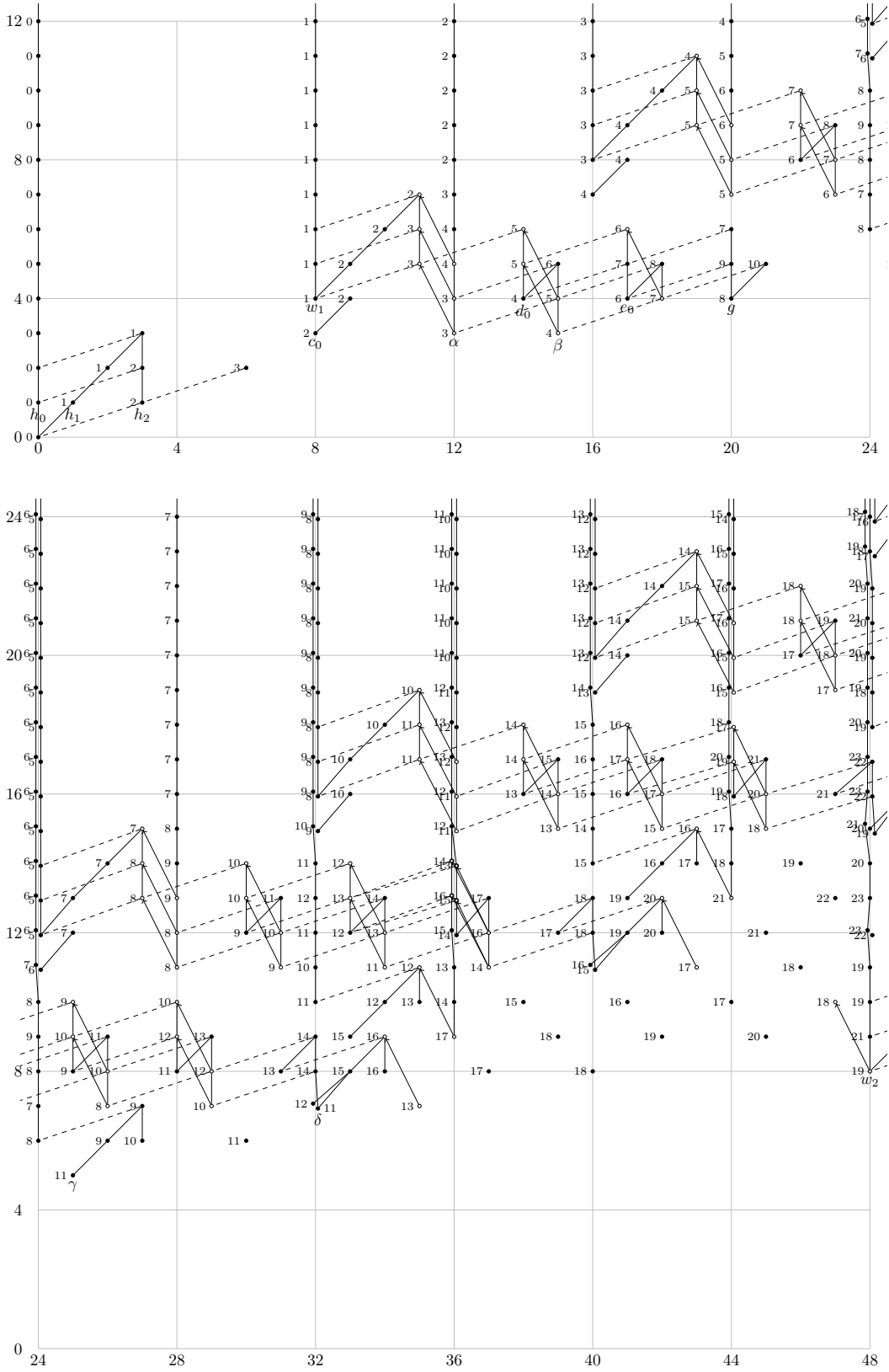
FIGURE 0.1. (E_2(tmf), d_2) for t - s \leq 48
