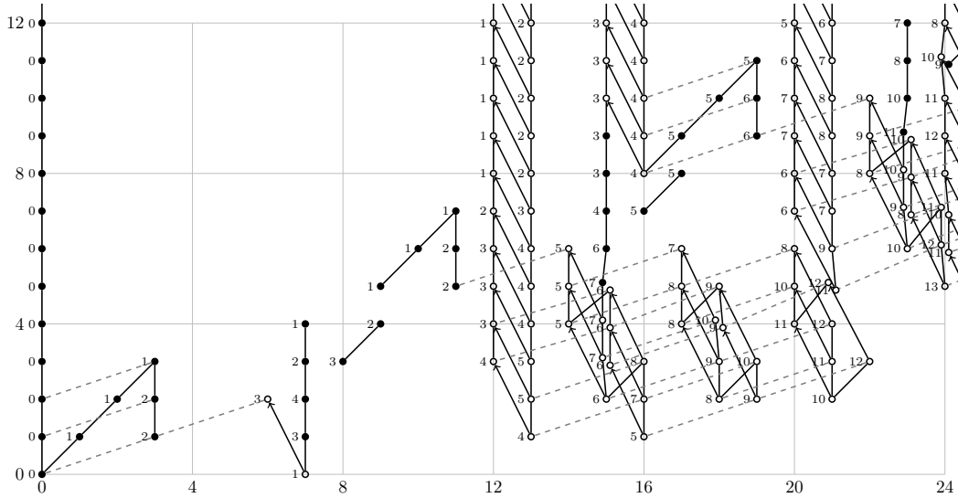
FIGURE 11.9. (E_2(j), d_2) for t - s \leq 24
