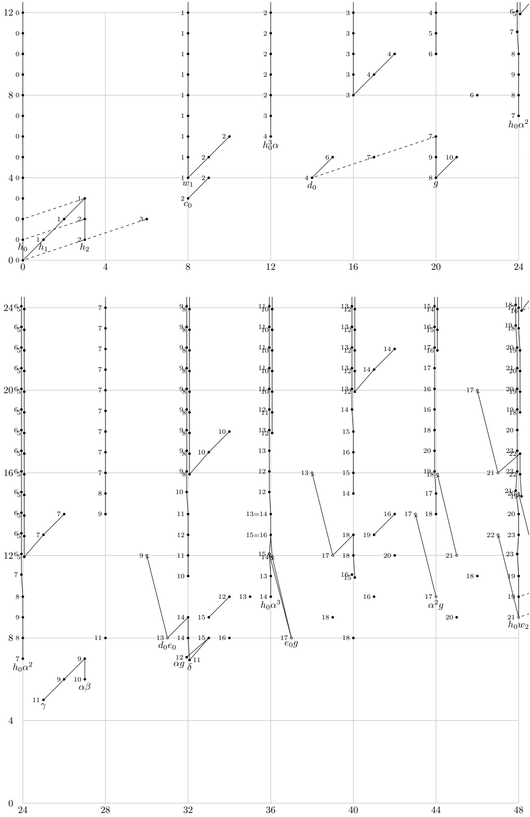
FIGURE 0.3. (E_4(tmf), d_4) for t - s \leq 48
