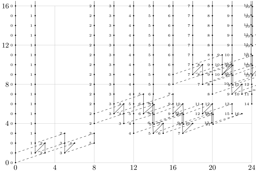
FIGURE 1.28. \text{Ext}_{A(2)}^{s,t}(M_2, \mathbb{F}_2) for 0 \leq t - s \leq 24
