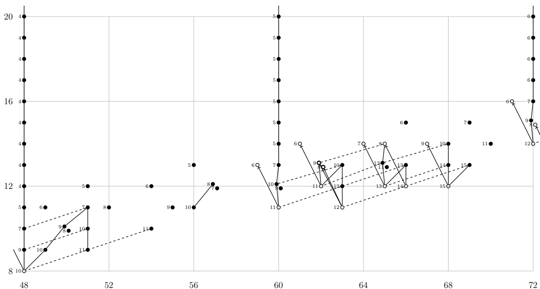
FIGURE 12.43. Hastened (E_r(tmf/B), d_r) for 48 \leq t - s \leq 72
