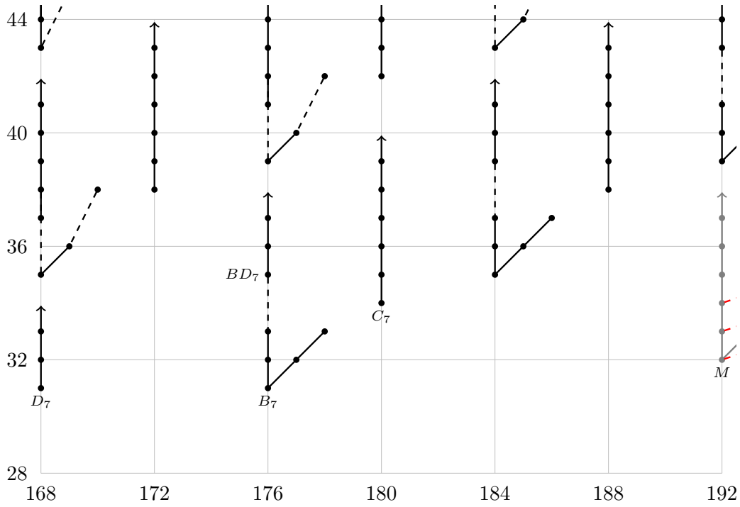
FIGURE 9.13. \pi_n(tmf) for 168 \leq n \leq 192
