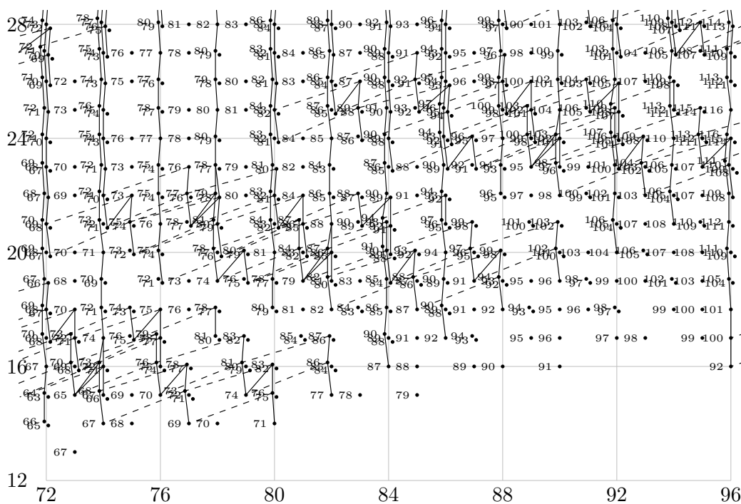
FIGURE 1.31. \text{Ext}_{A(2)}^{s,t}(M_2, \mathbb{F}_2) for 72 \leq t - s \leq 96
