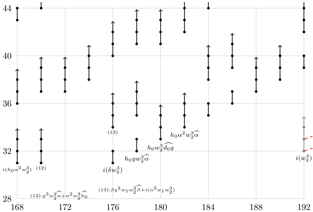
FIGURE 7.8. E_4(tm\mathbf{f}/\eta) = E_\infty(tm\mathbf{f}/\eta) for 168 \leq t - s \leq 192
