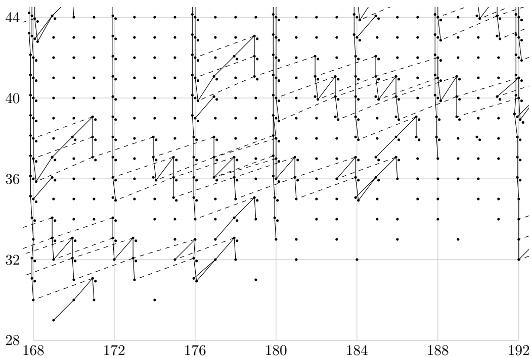
FIGURE 1.18. \text{Ext}_{A(2)}^{s,t}(\mathbb{F}_2, \mathbb{F}_2) for 168 \leq t - s \leq 192
