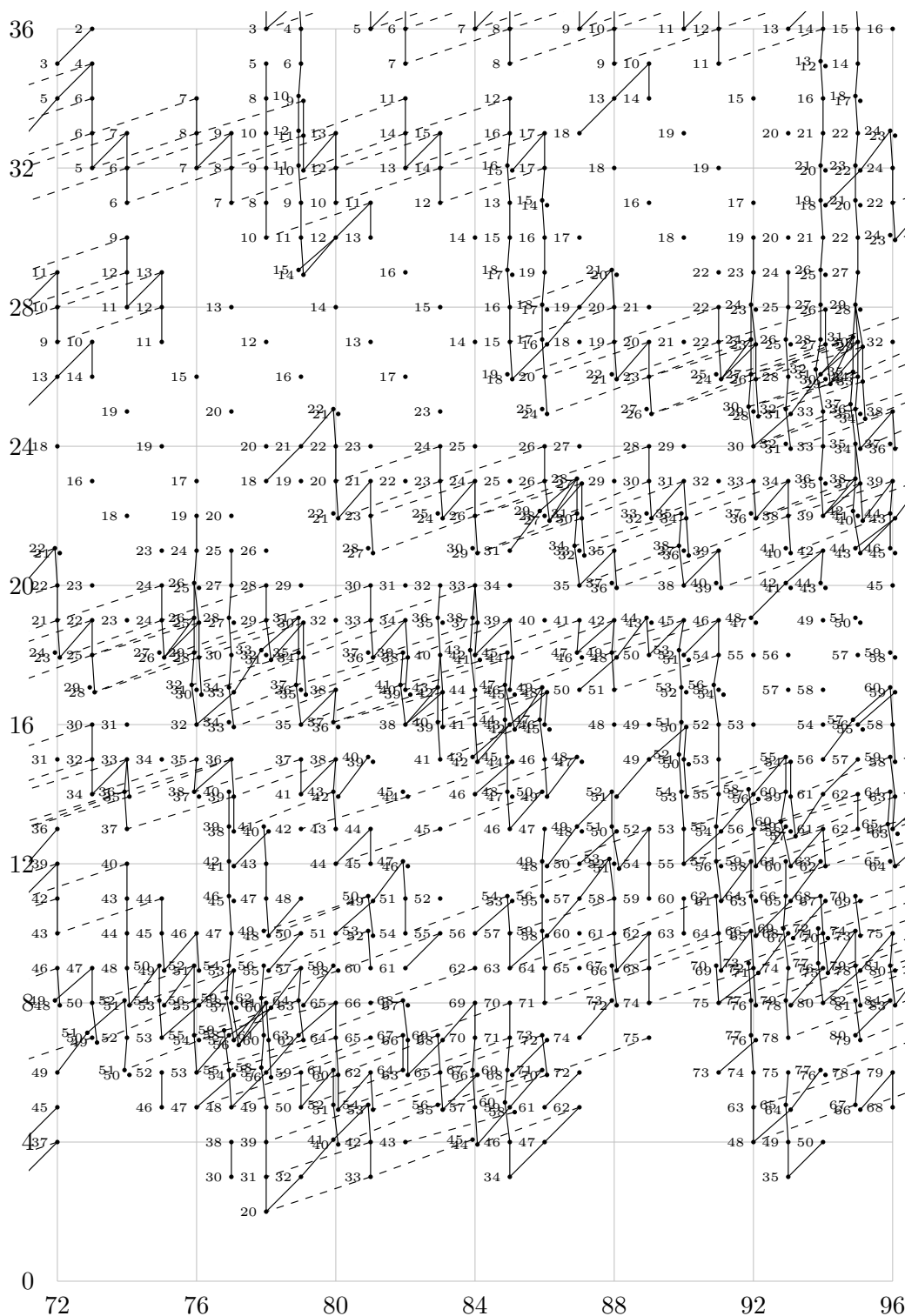
FIGURE 1.4. \text{Ext}_A^{s,t}(\mathbb{F}_2, \mathbb{F}_2) for 72 \leq t - s \leq 96
