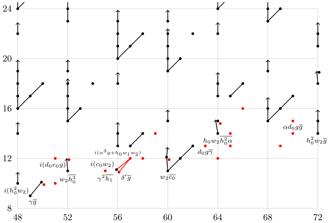
FIGURE 8.3. E_5(tm\mathbf{f}/\nu) = E_\infty(tm\mathbf{f}/\nu) for 48 \leq t - s \leq 72
