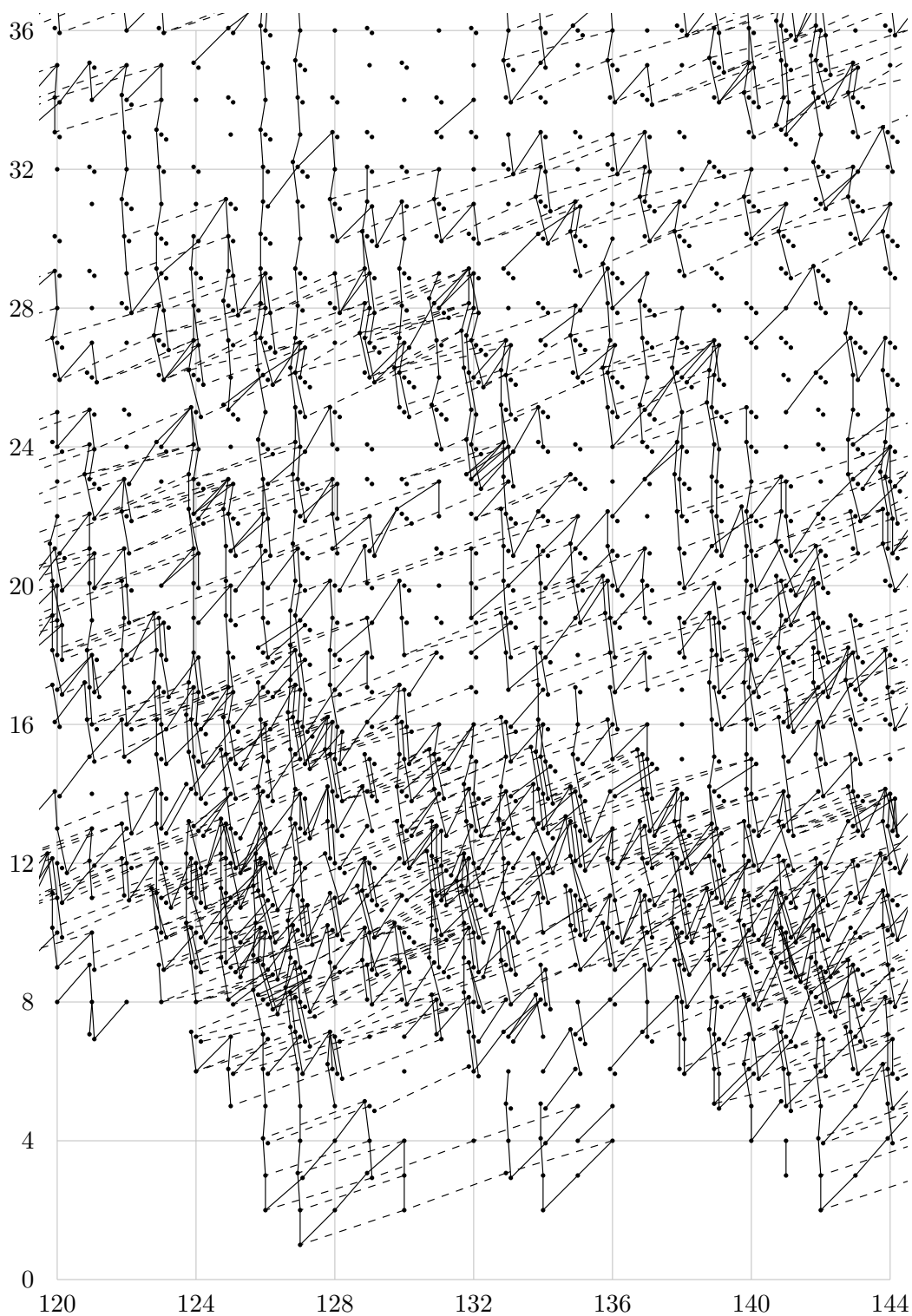
FIGURE 1.6. \text{Ext}_A^{s,t}(\mathbb{F}_2, \mathbb{F}_2) for 120 \leq t - s \leq 144
