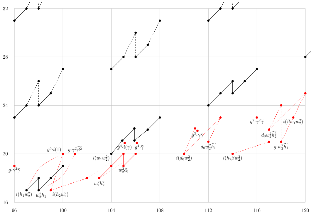
FIGURE 12.5. E_\infty(tmf/2) for 96 \leq t - s \leq 120 , with all hidden 2-, \eta - and \nu -extensions
