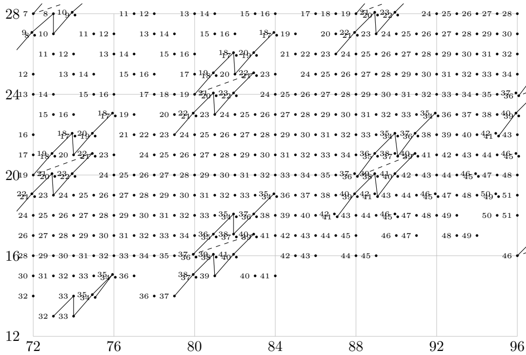
FIGURE 1.27. \text{Ext}_{A(2)}^{s,t}(M_1, \mathbb{F}_2) for 72 \leq t - s \leq 96
