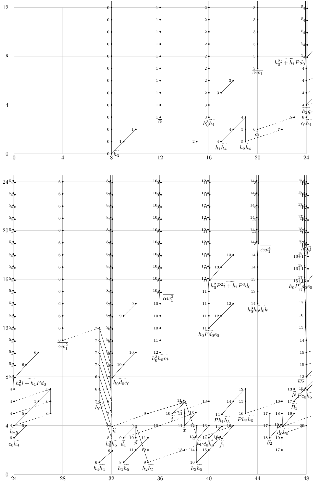
FIGURE 11.28. (E_3(tm\mathbb{f}/S), d_3) for t - s \leq 48
