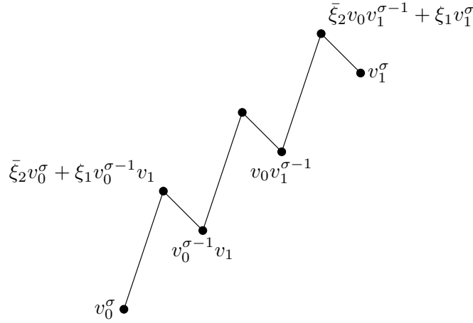
FIGURE 3.1. The syzygy \Omega_{E(1)_*}^\sigma(\mathbb{F}_2) for \sigma = 3
