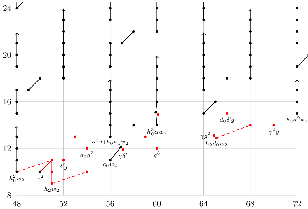
FIGURE 5.3. E_5(tm) = E_\infty(tm) for 48 \leq t - s \leq 72
