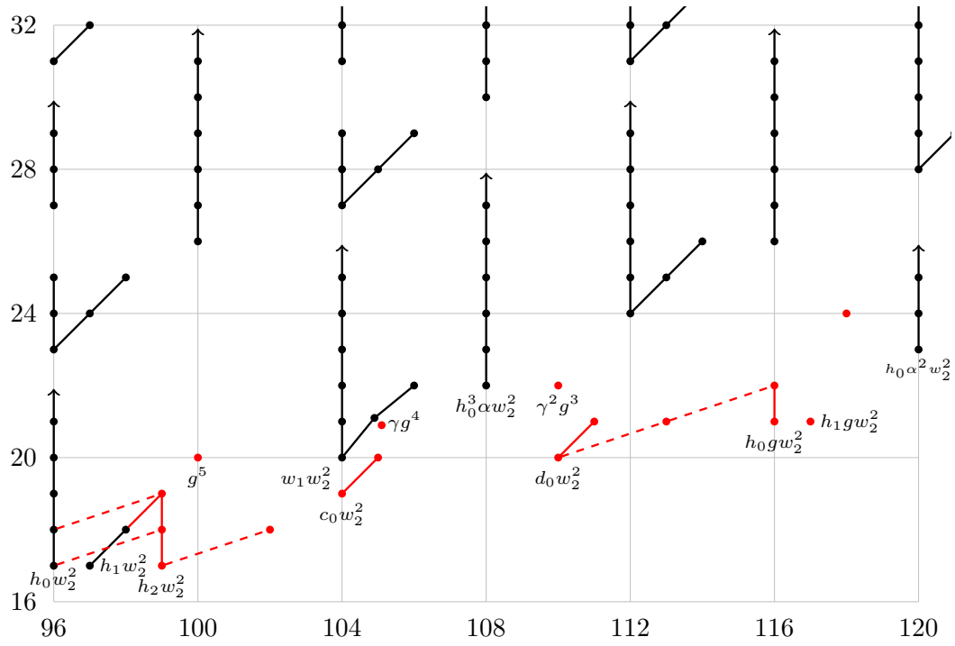
FIGURE 5.5. E_5(tm\mathbb{f}) = E_\infty(tm\mathbb{f}) for 96 \leq t - s \leq 120
