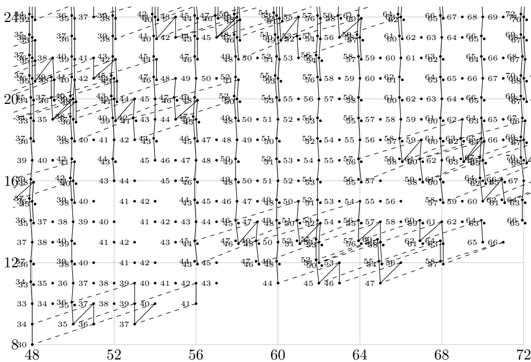
FIGURE 1.30. \text{Ext}_{A(2)}^{s,t}(M_2, \mathbb{F}_2) for 48 \leq t - s \leq 72
