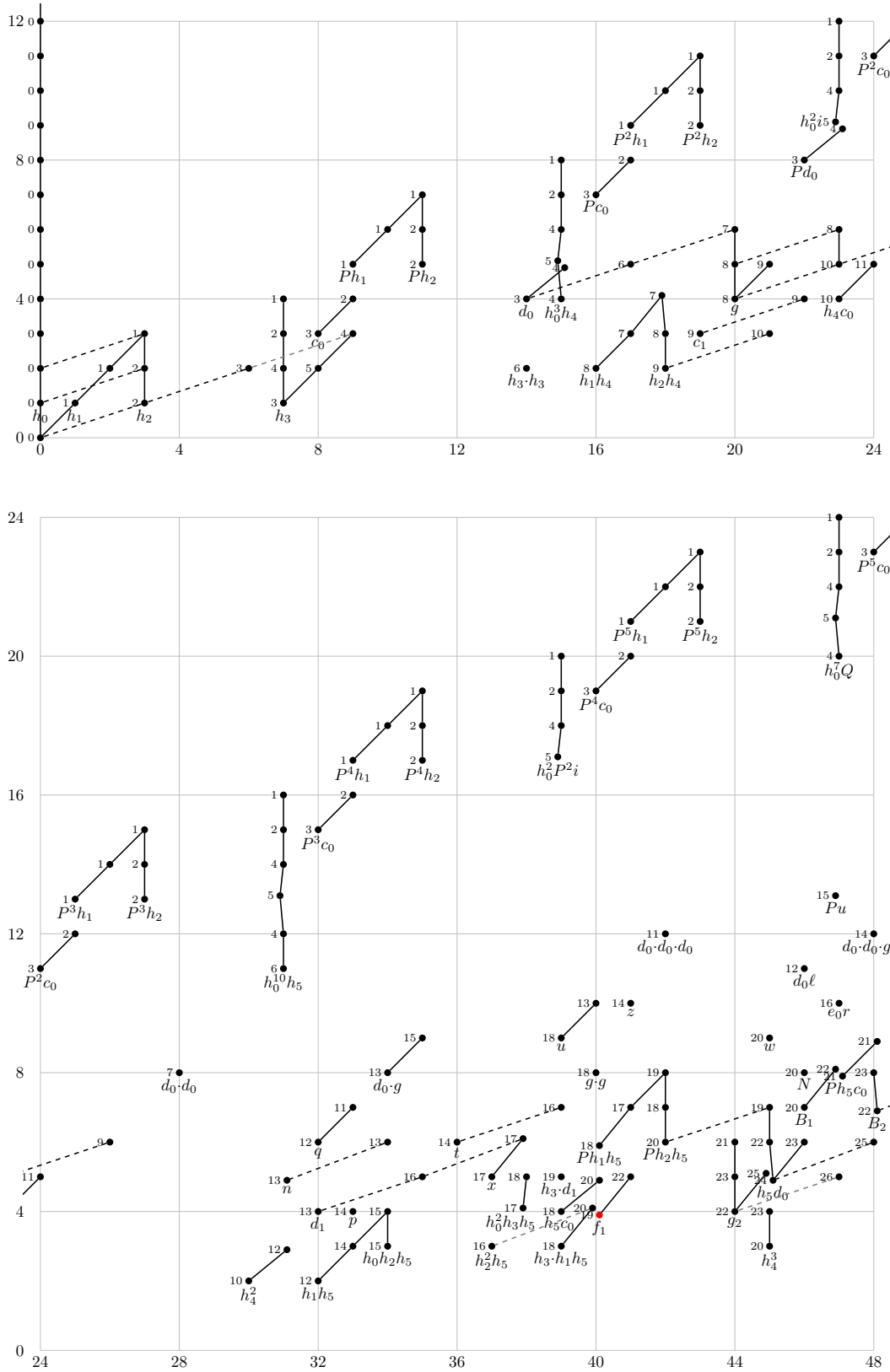
FIGURE 11.13. E_5(S) = E_\infty(S) for t - s \leq 48
