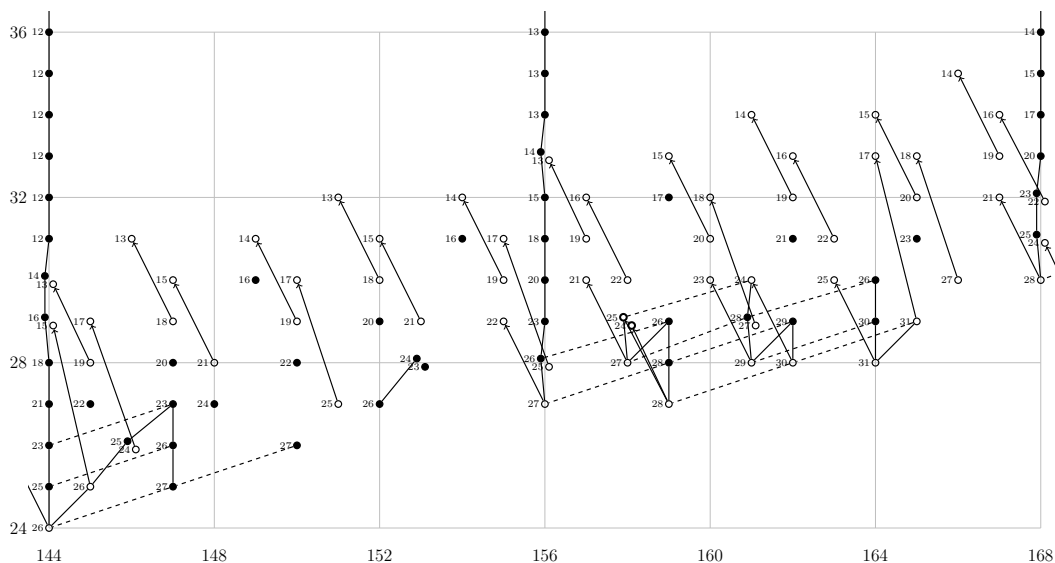
FIGURE 12.47. Hastened (E_r(tmf/B), d_r) for 144 \leq t - s \leq 168
