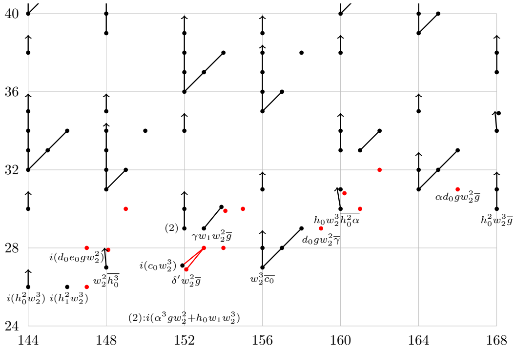
FIGURE 8.7. E_5(tm\mathbf{f}/\nu) = E_\infty(tm\mathbf{f}/\nu) for 144 \leq t - s \leq 168
