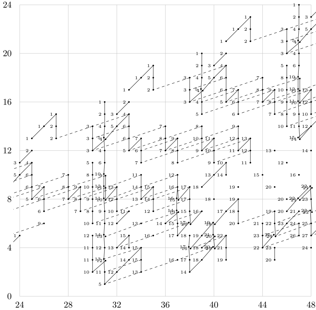
FIGURE 1.2. \text{Ext}_A^{s,t}(\mathbb{F}_2, \mathbb{F}_2) for 24 \leq t - s \leq 48
