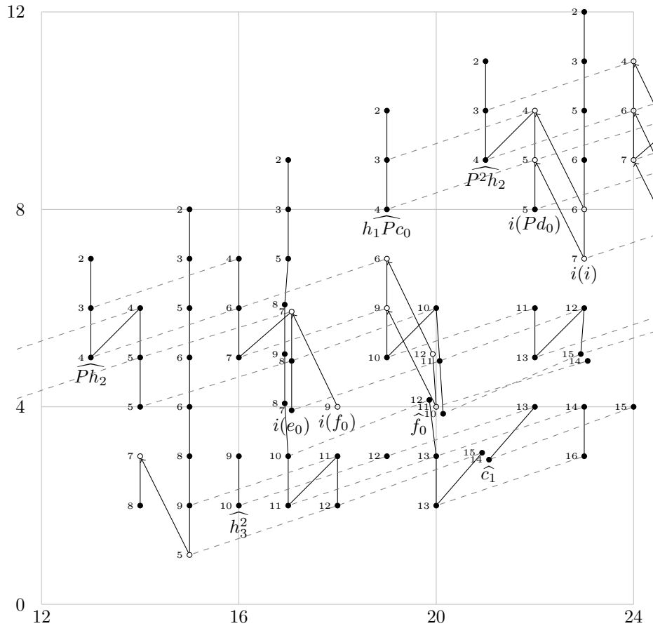
FIGURE 11.22. (E_2(C\eta), d_2) for 12 \leq t - s \leq 24
