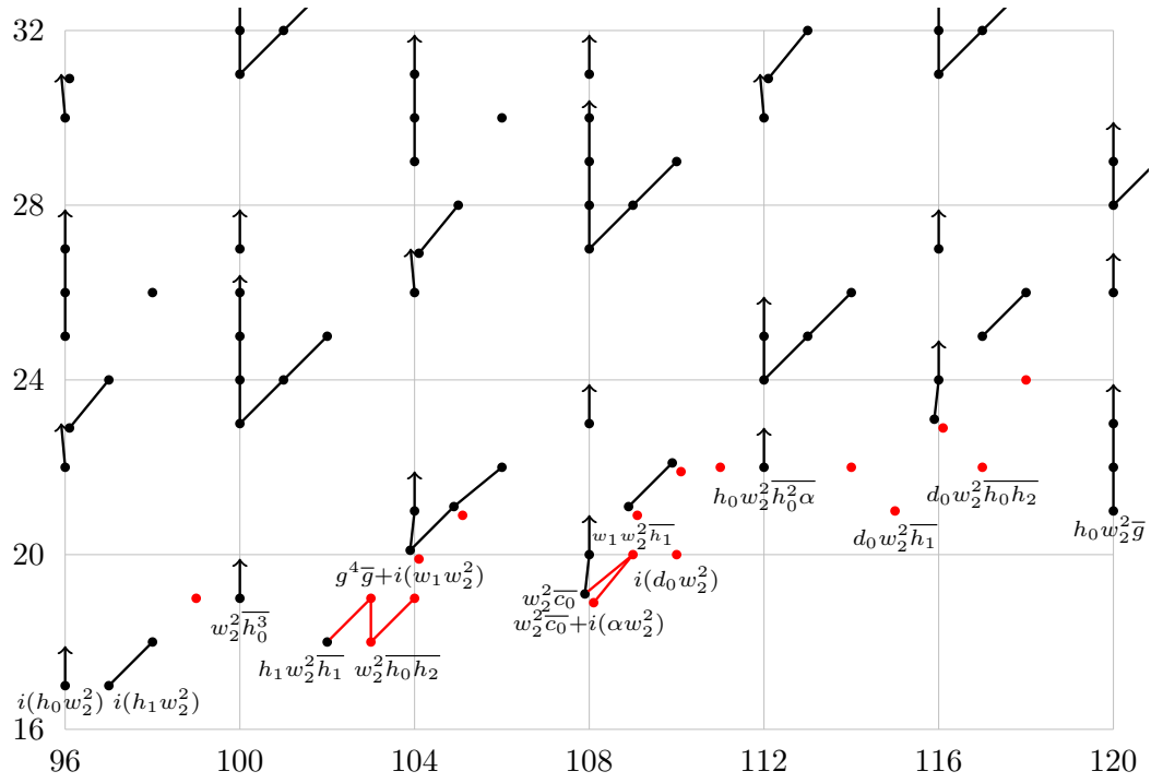
FIGURE 8.5. E_5(tm\mathbb{f}/\nu) = E_\infty(tm\mathbb{f}/\nu) for 96 \leq t - s \leq 120
