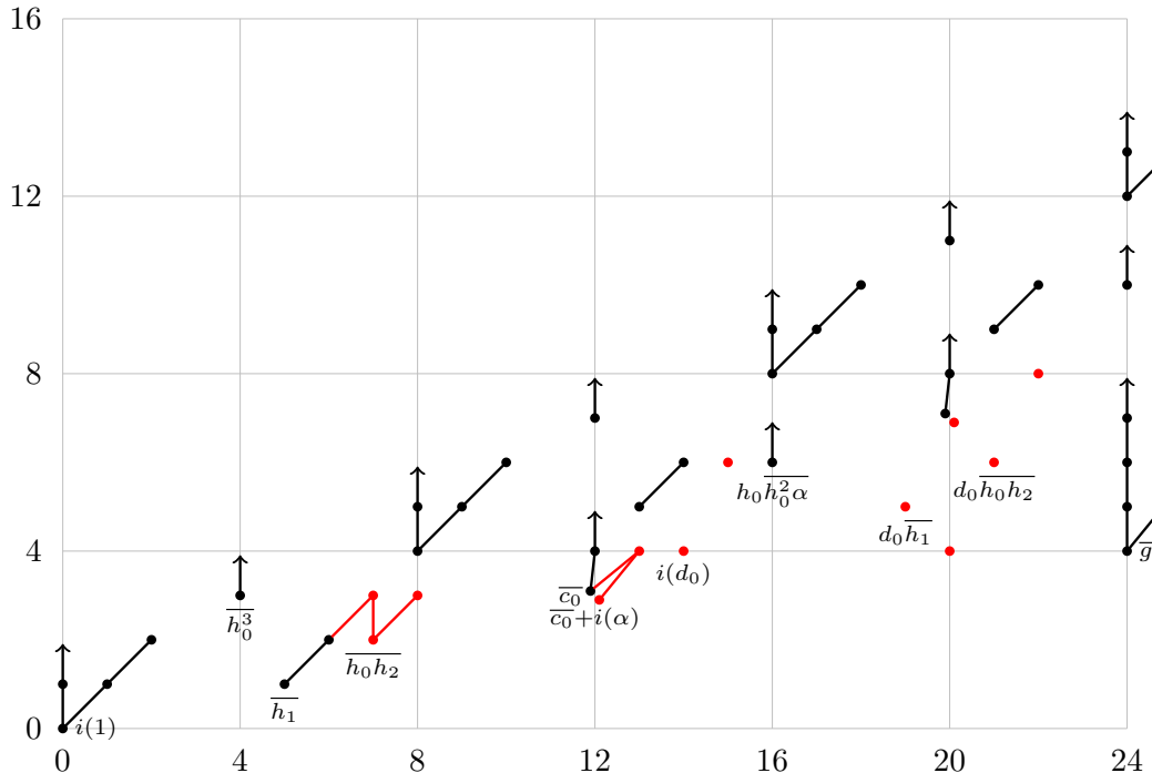
FIGURE 8.1. E_5(tm\mathbb{f}/\nu) = E_\infty(tm\mathbb{f}/\nu) for 0 \leq t - s \leq 24
