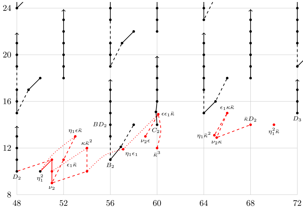
FIGURE 9.8. \pi_n(tmf) for 48 \leq n \leq 72
