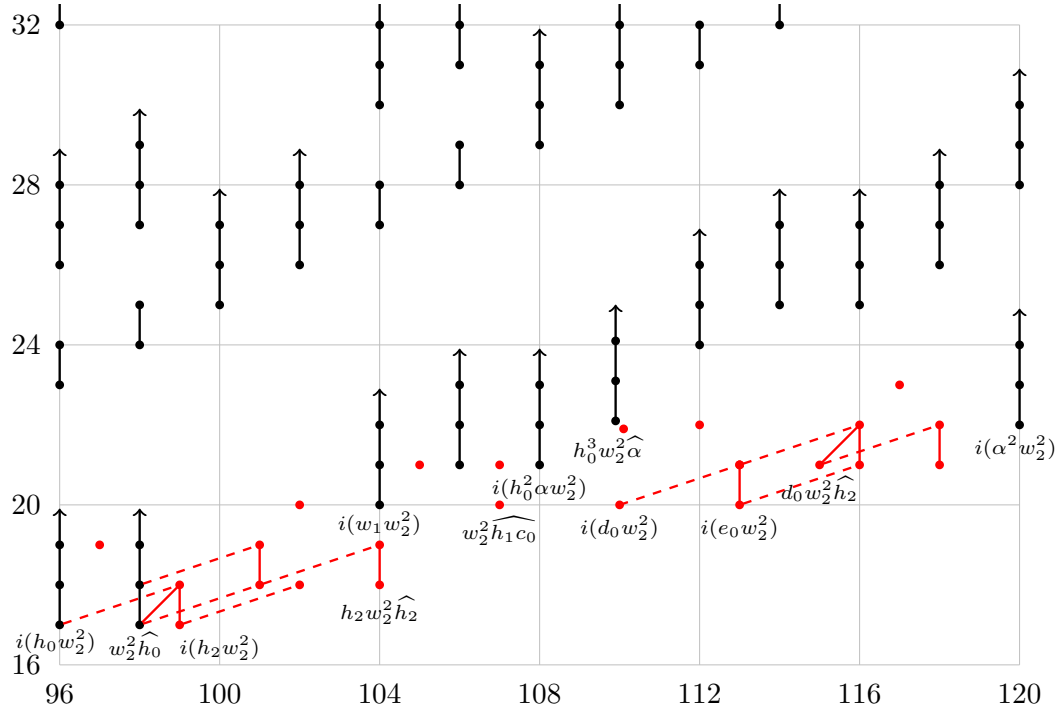
FIGURE 7.5. E_4(tmf/\eta) = E_\infty(tmf/\eta) for 96 \leq t - s \leq 120
