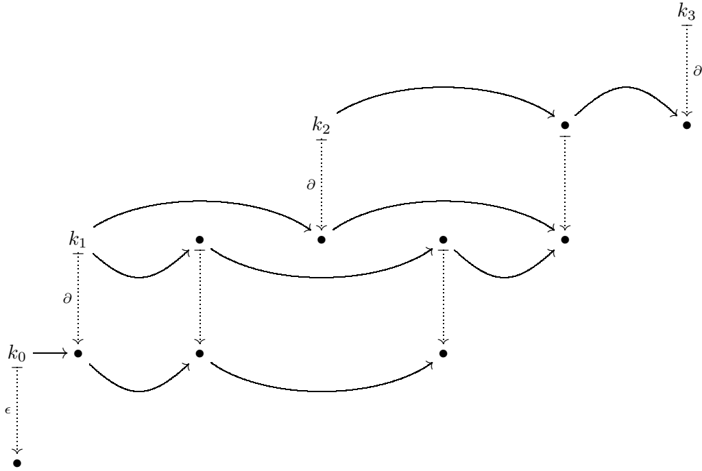
FIGURE 1.22. A 3-fold extension K_* representing c_0
