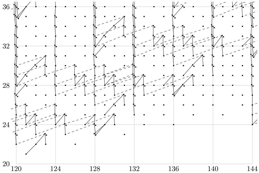
FIGURE 1.16. \text{Ext}_{A(2)}^{s,t}(\mathbb{F}_2, \mathbb{F}_2) for 120 \leq t - s \leq 144
