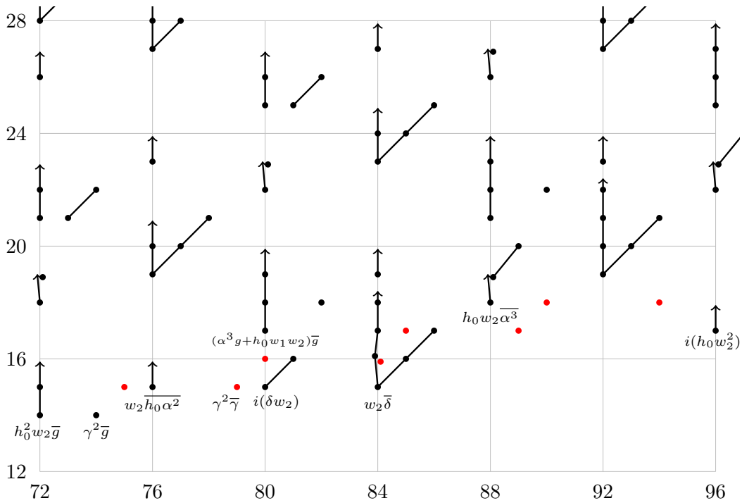
FIGURE 8.4. E_5(tm\mathbf{f}/\nu) = E_\infty(tm\mathbf{f}/\nu) for 72 \leq t - s \leq 96
