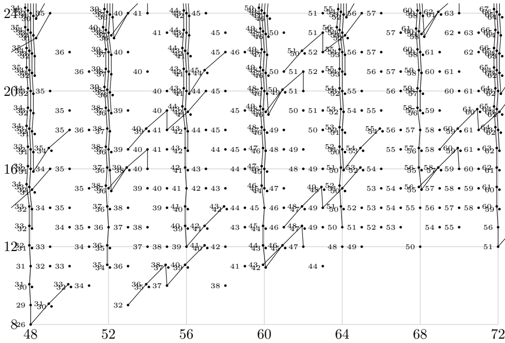
FIGURE 1.34. \text{Ext}_{A(2)}^{s,t}(M_4, \mathbb{F}_2) for 48 \leq t - s \leq 72
