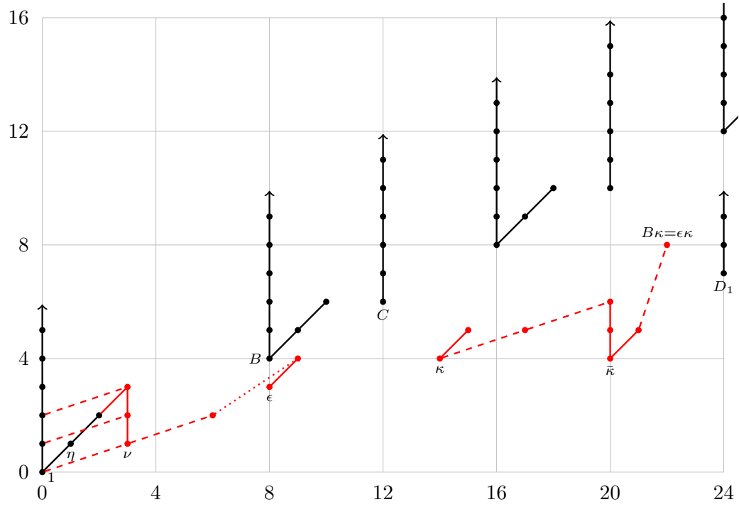
FIGURE 9.6. \pi_n(tmf) for 0 \leq n \leq 24
