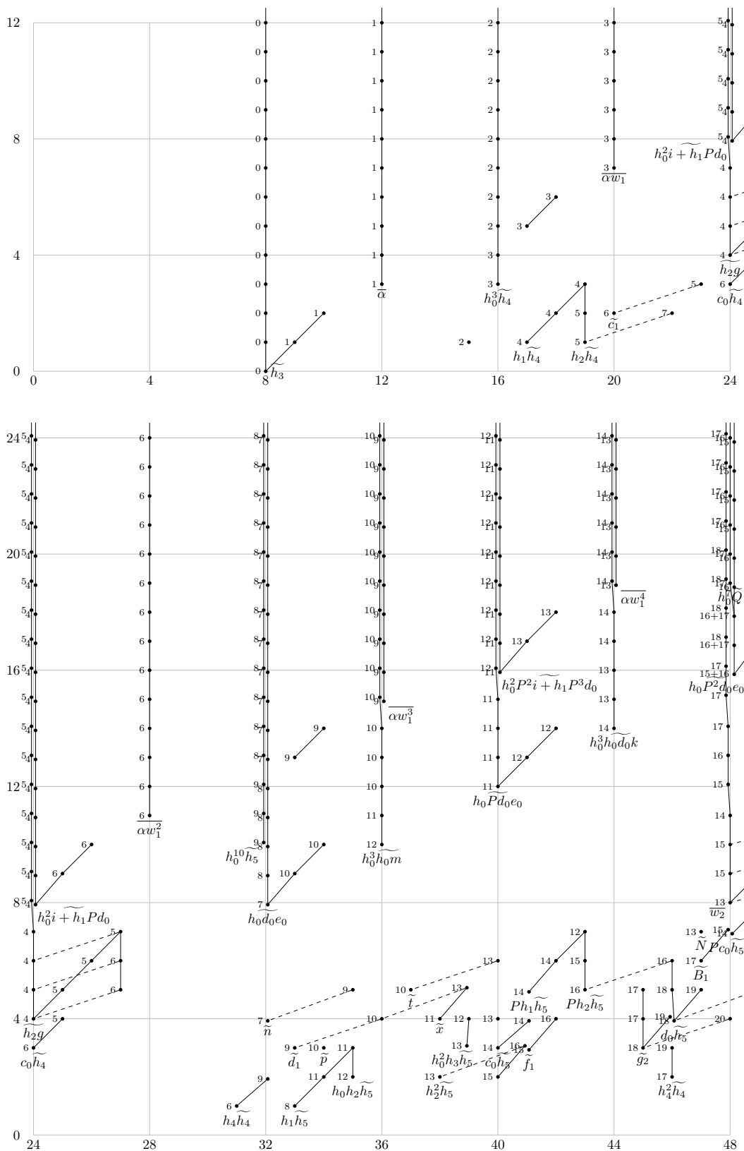
FIGURE 11.30. E_5(tm\mathbb{f}/S) = E_\infty(tm\mathbb{f}/S) for t - s \leq 48
