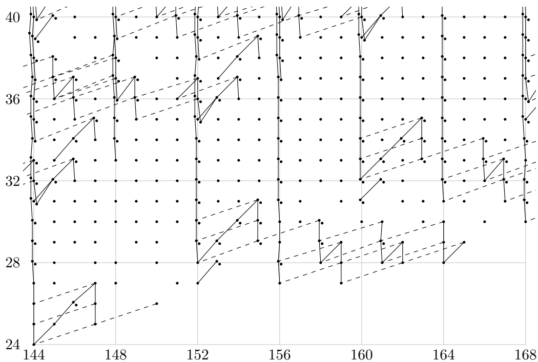
FIGURE 1.17. \text{Ext}_{A(2)}^{s,t}(\mathbb{F}_2, \mathbb{F}_2) for 144 \leq t - s \leq 168
