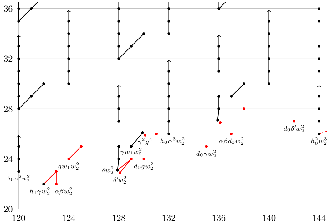
FIGURE 5.6. E_5(tm\mathbb{f}) = E_\infty(tm\mathbb{f}) for 120 \leq t - s \leq 144
