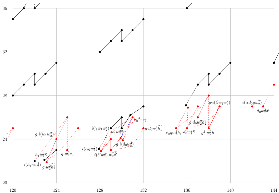
FIGURE 12.6. E_\infty(tmf/2) for 120 \leq t - s \leq 144 , with all (potential) hidden 2-, \eta - and \nu -extensions
