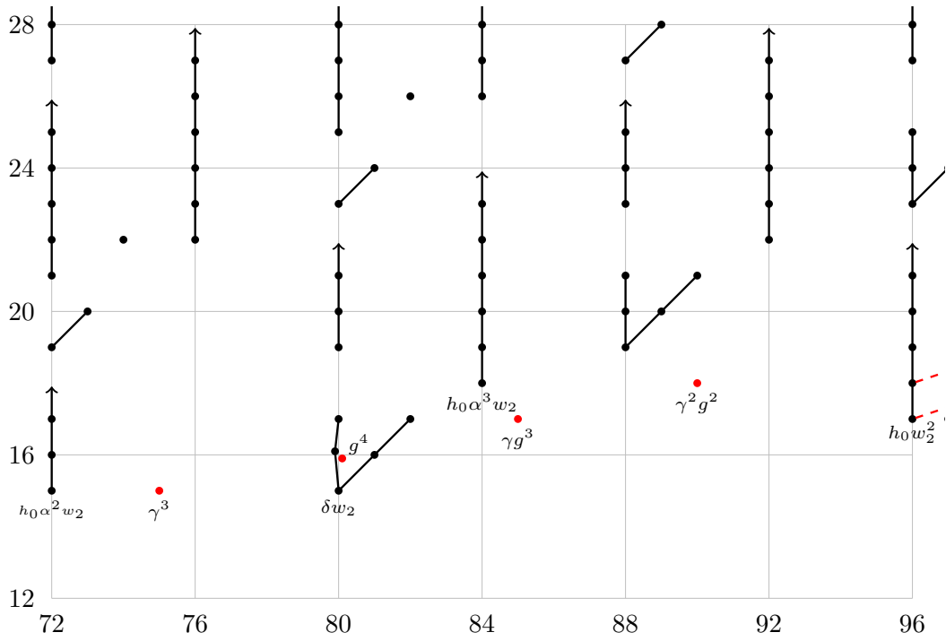
FIGURE 5.4. E_5(tm) = E_\infty(tm) for 72 \leq t - s \leq 96
