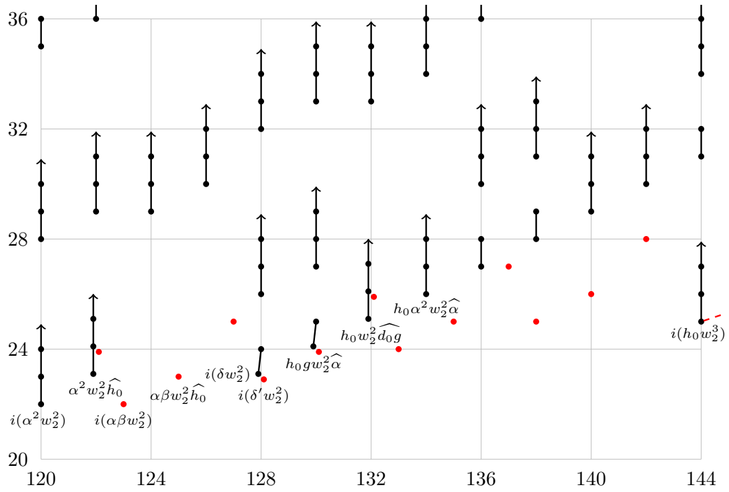
FIGURE 7.6. E_4(tmf/\eta) = E_\infty(tmf/\eta) for 120 \leq t - s \leq 144
