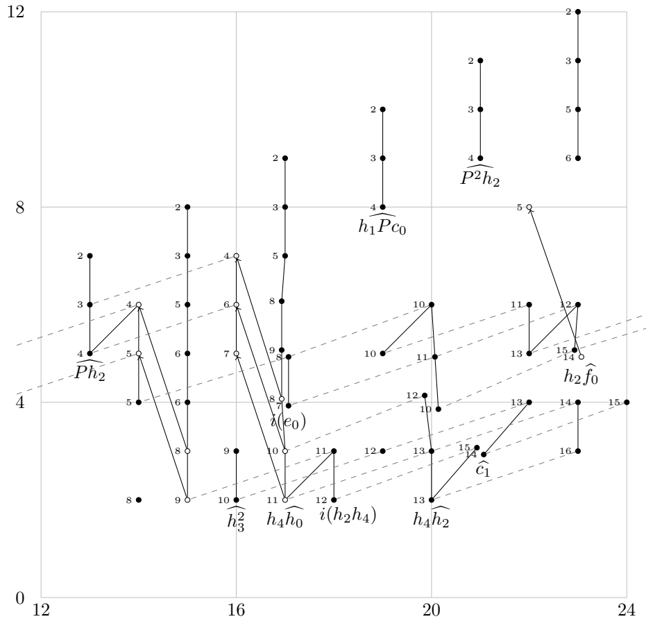
FIGURE 11.23. (E_3(C\eta), d_3) for 12 \leq t - s \leq 24
