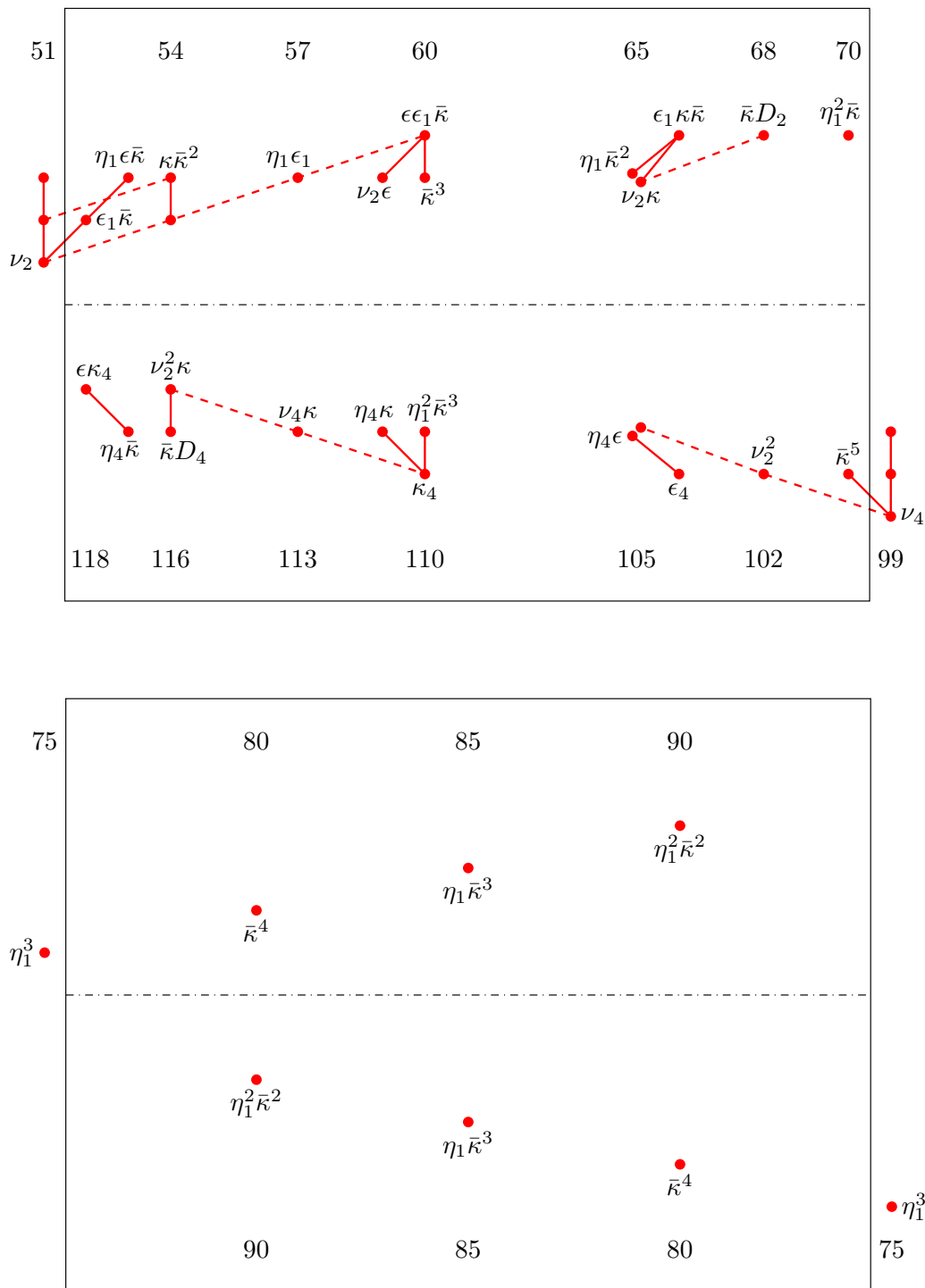
FIGURE 10.2. The self-dual submodule \Theta\pi_n(tmf) \subset \Gamma_B\pi_n(tmf) for 52 \leq n, 170 - n \leq 94 , with \eta_1 \bar{\kappa}^4 = \eta_4 \epsilon_4 + \nu^2 \nu_4 and \bar{\kappa}^5 = \eta_1^4
