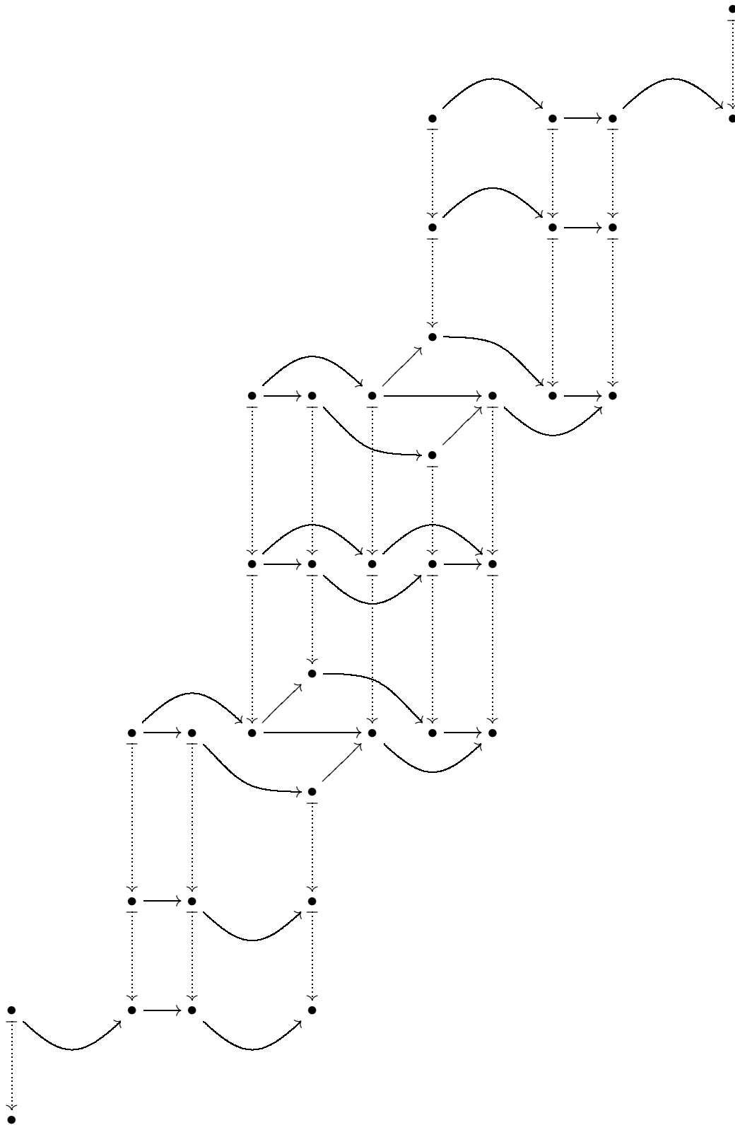
FIGURE 2.4. Spliced A(1) -extensions
