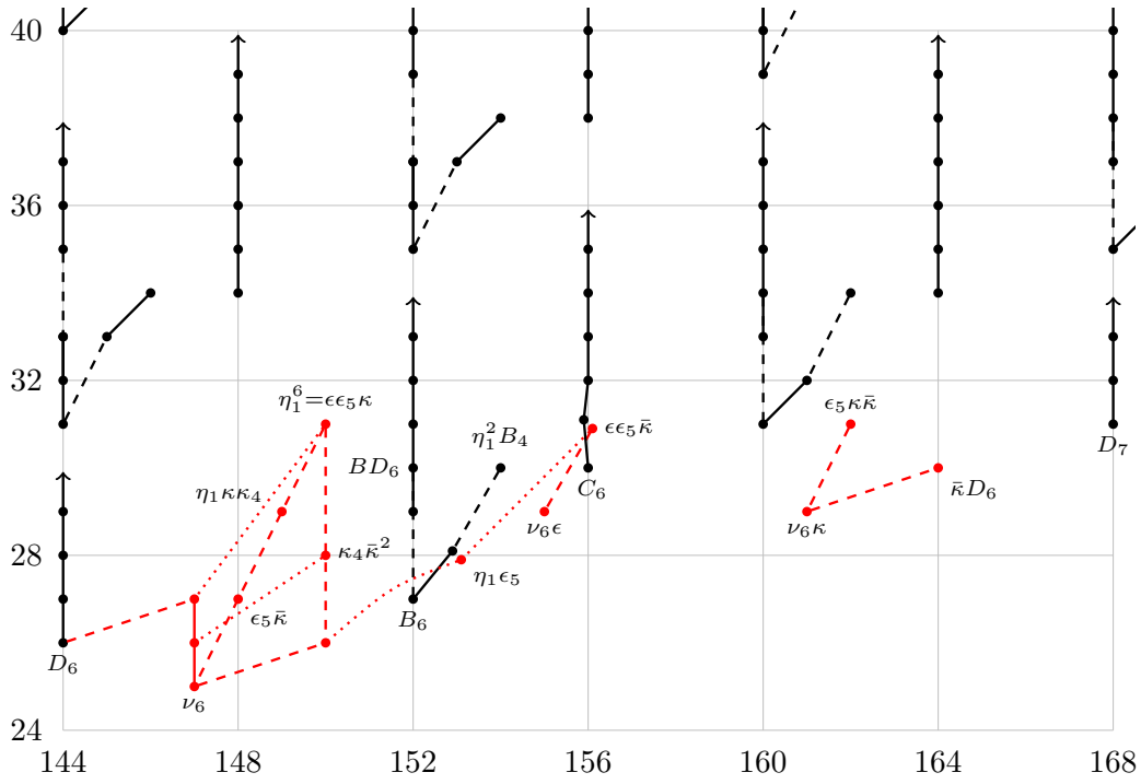
FIGURE 9.12. \pi_n(tmf) for 144 \leq n \leq 168
