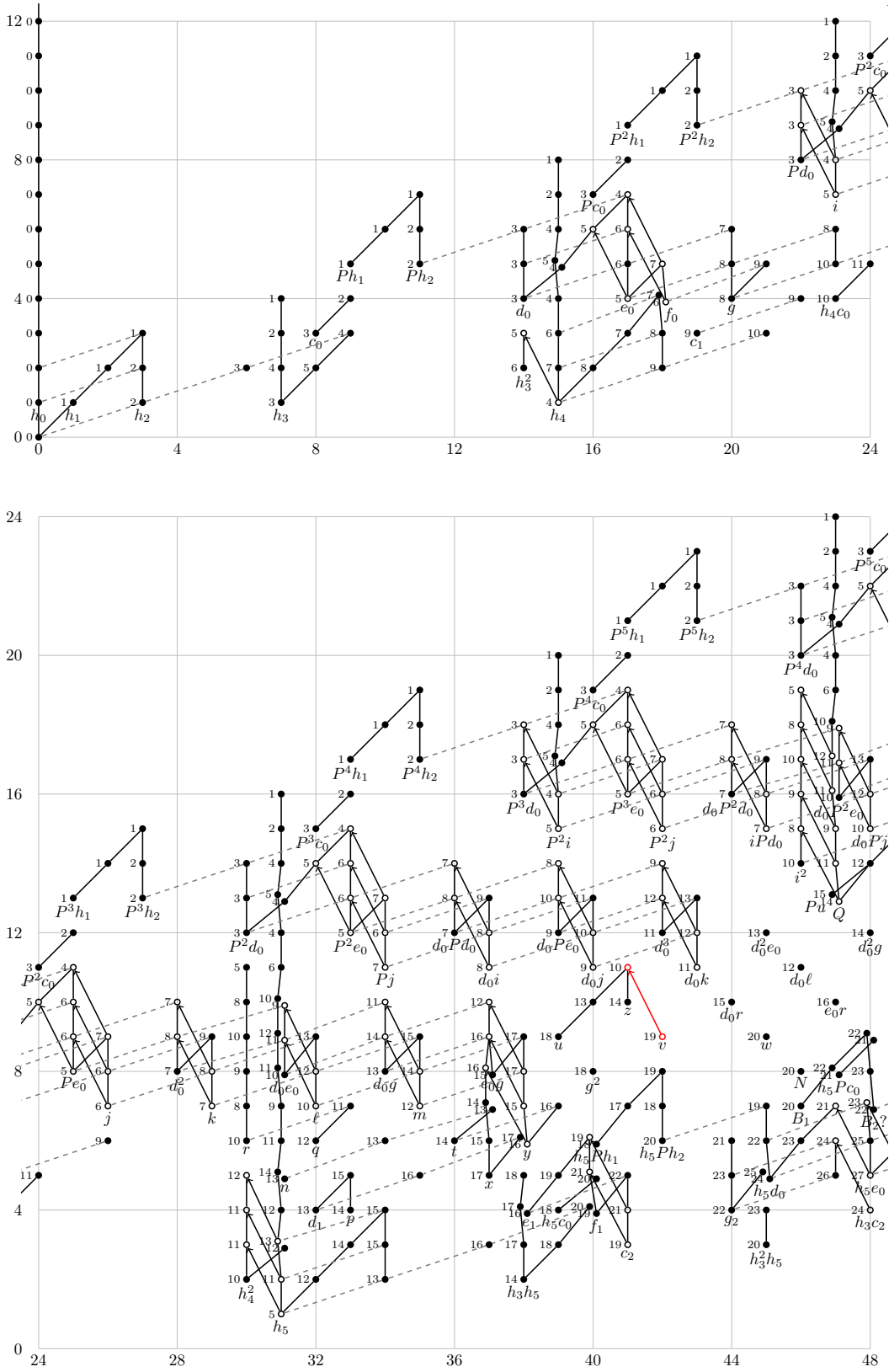
FIGURE 11.10. (E_2(S), d_2) for t - s \leq 48
