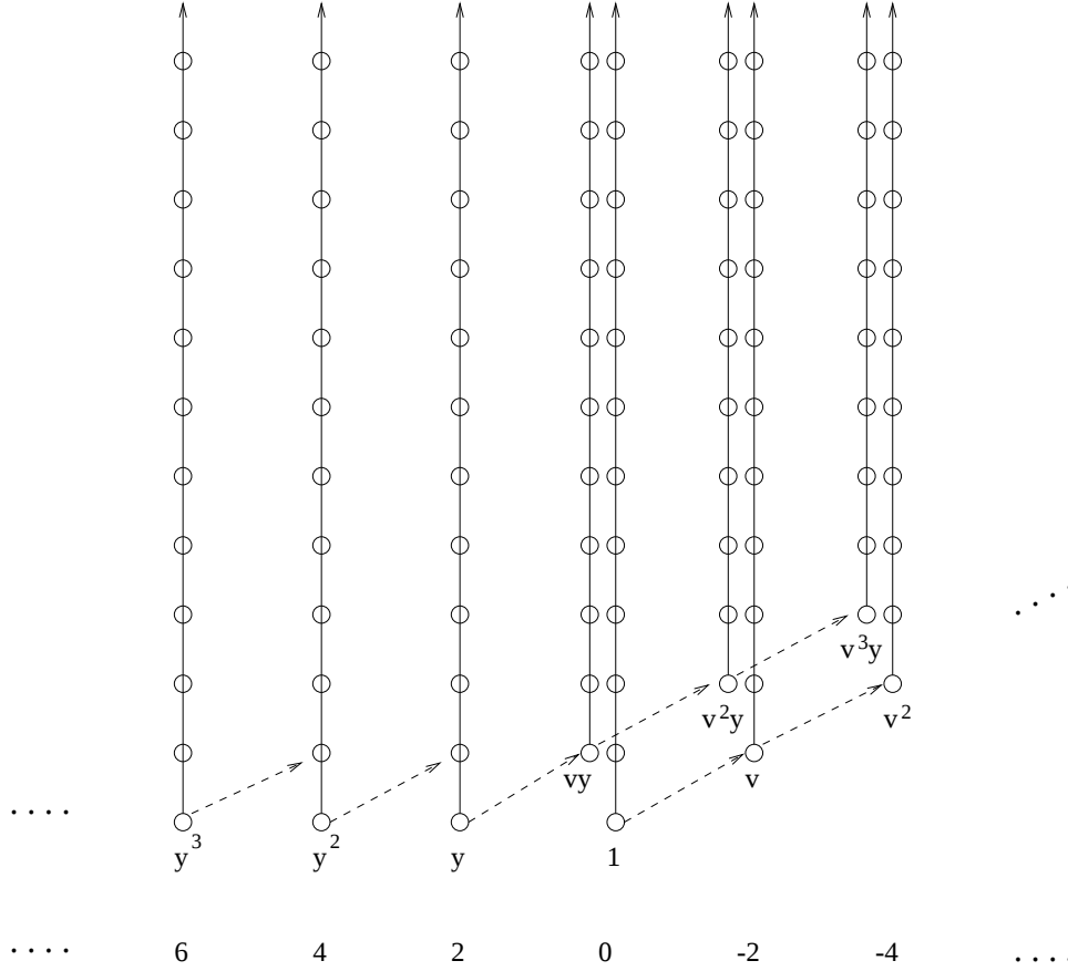
FIGURE 2.5. The Adams spectral sequence for ku^*(BC_2) .
