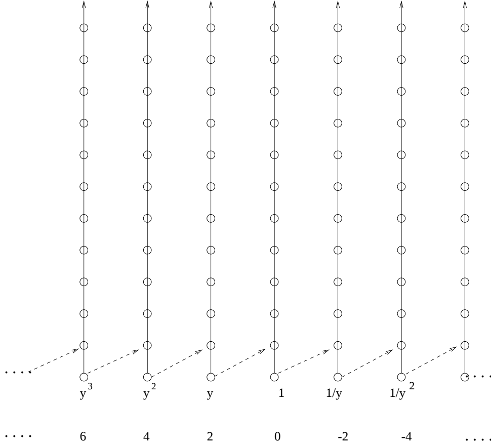
FIGURE 3.2. t(ku)_{C_2}^* = \mathbb{Z}_2^\wedge[y, 1/y] with v = 2/y
