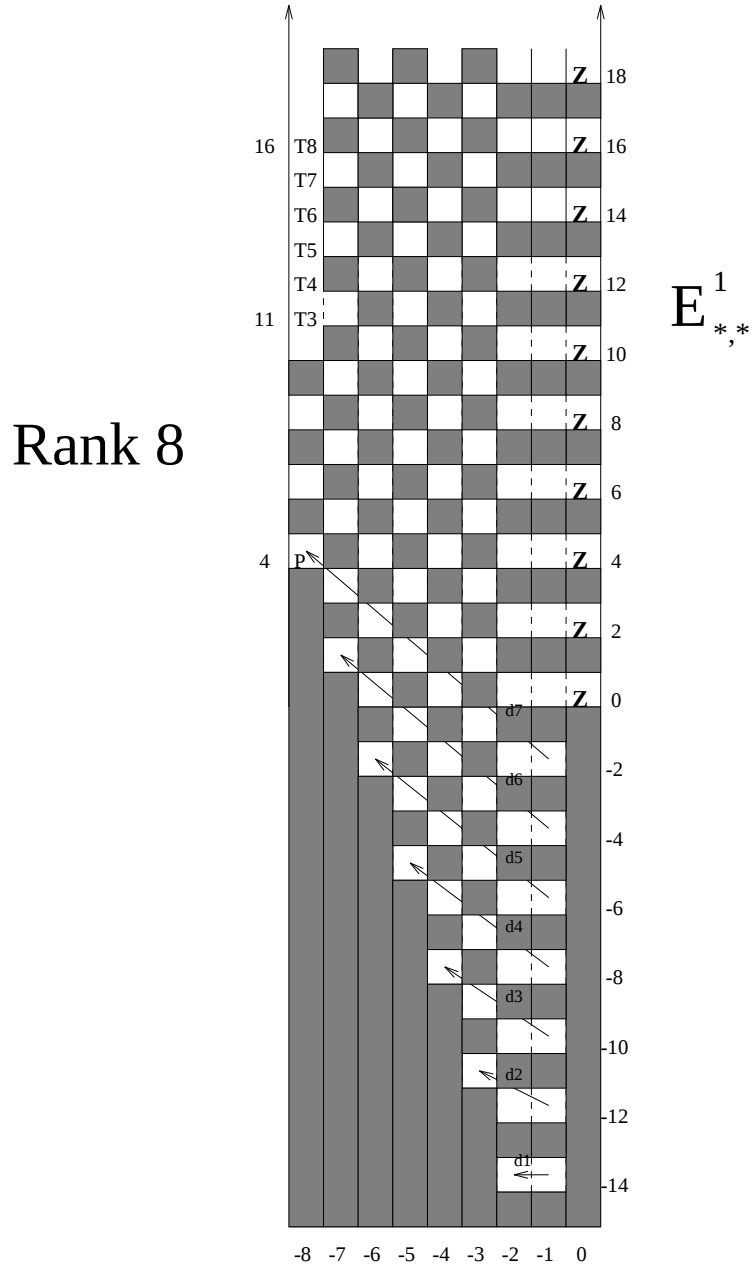
FIGURE 4.6. The local cohomology spectral sequence for ku_*(BV) with V of rank 8. The (-1) st and (-2) nd columns start in degrees -2r + 2 . After this, the start increases in steps of 3. The bottom nonzero entry of the (-r) th column is in degree r - 4 (coming from H_r^r(T_r) = P^\vee(r - 4) ). The subsequent contributions are \text{Start}(r + 3)T_3^\vee , \text{Start}(r + 4)T_4^\vee , \dots , \text{Start}(2r)T_r^\vee = P^\vee(2r) . In the picture, the differential d^i connects the lowest nonzero groups in their respective columns on the E^i -page.
