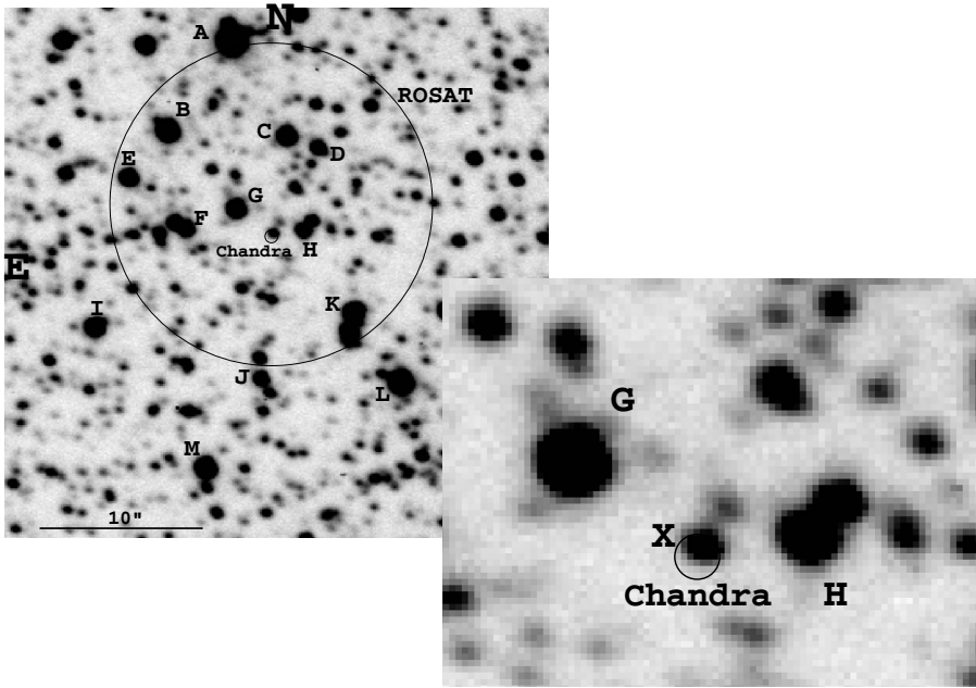
Fig. 1. A Magellan I image of the ROSAT error box (10 arcsec radius) of KS 1731–260 ( left ) and a close-up of the Chandra position (0.4 arcsec) with star “X” as our proposed optical and infrared counterpart ( right ). Star labeling is as in Barret et al. (1998). North is upwards and east is to the left.
