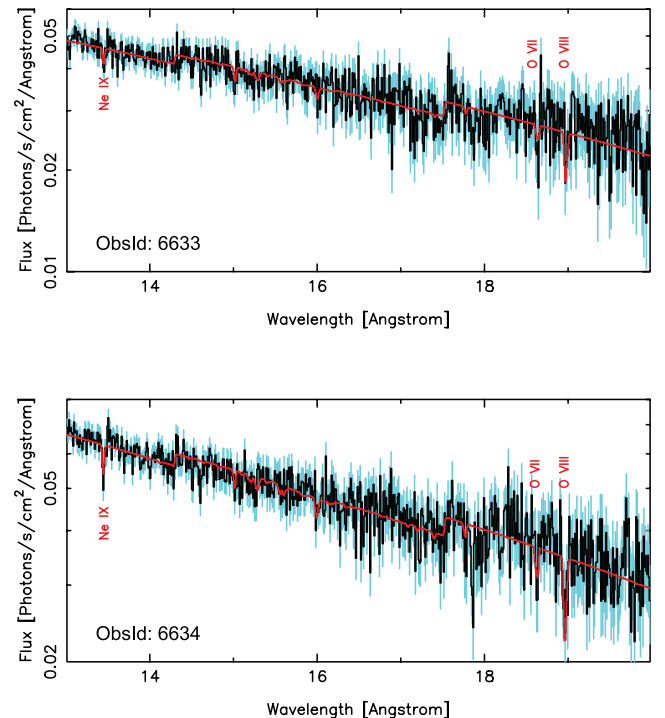
FIG. 2.—Best-fitting XSTAR photoionization models for ObsID 6633 (top) and 6634 (bottom). The Ne IX, O VII, and O VIII lines are reproduced well by the models.
