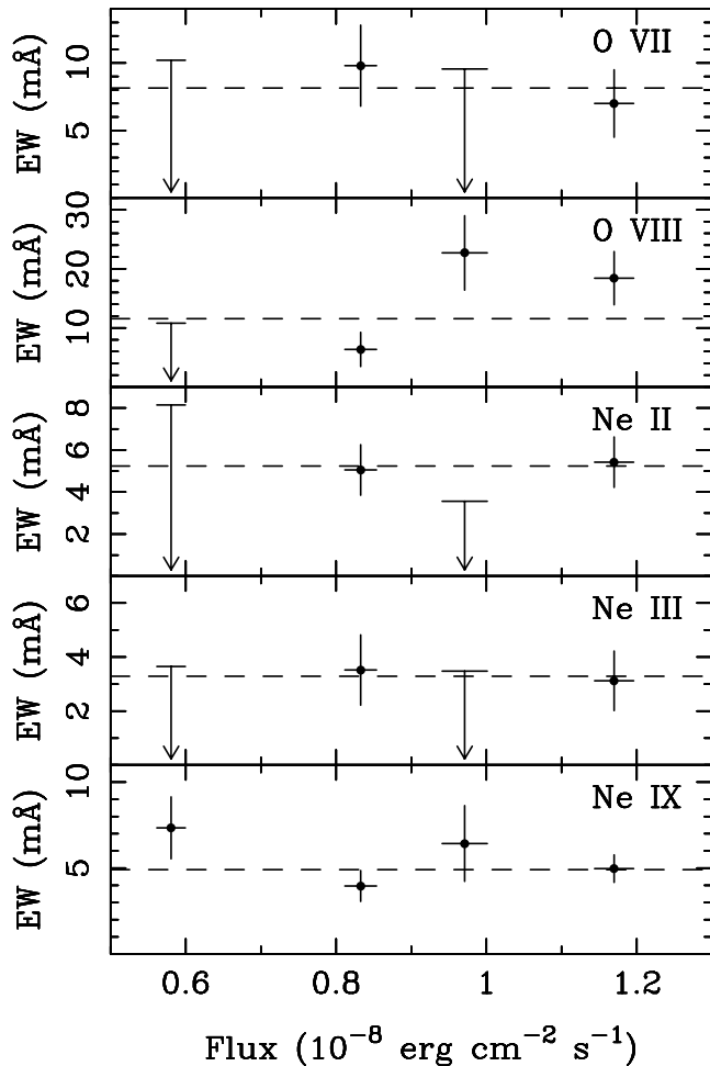
FIG. 4.—Equivalent widths (mÅ) of the various absorption lines in 4U 1820–30 vs. 0.5–10 keV unabsorbed source flux in units of 10^{-8} ergs \text{cm}^{-2} \text{s}^{-1} . Dashed lines indicate the weighted mean of the measured equivalent widths. Arrows indicate 95% confidence upper limits, and error bars indicate 1\sigma uncertainties.
