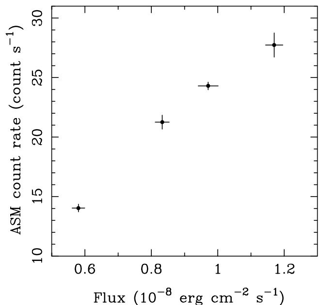
FIG. 3.—Plot of 0.5–10 keV unabsorbed source flux determined from fitting to the HEG spectra shown vs. the 1 day average RXTE All-Sky Monitor count rate on the day of each observation.
