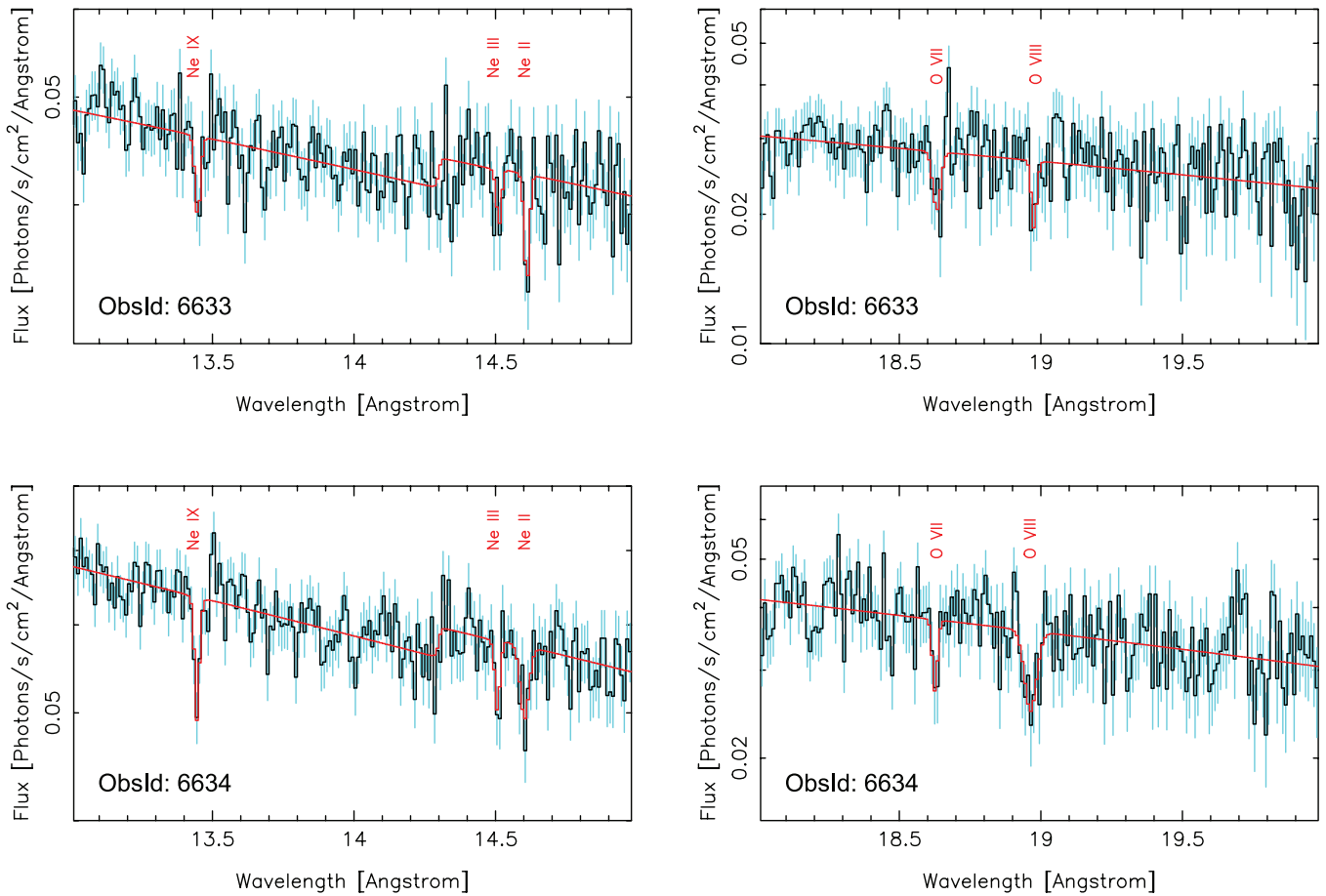
FIG. 1.— Segments of the combined first-order MEG spectra of 4U 1820–30 at 13–15 and 18–20 Å. For illustrative purposes the data have been rebinned by a factor of 2. The top panels show these regions in ObsID 6633, and the bottom panels show these regions in ObsID 6634. The data are in black, and the 1\sigma error bars are in blue. The best-fitting model is in red. The continuum is fit by a power law modified by neutral ISM absorption edges, where appropriate. Absorption lines are modeled by a Gaussian. Table 2 gives the line properties.
