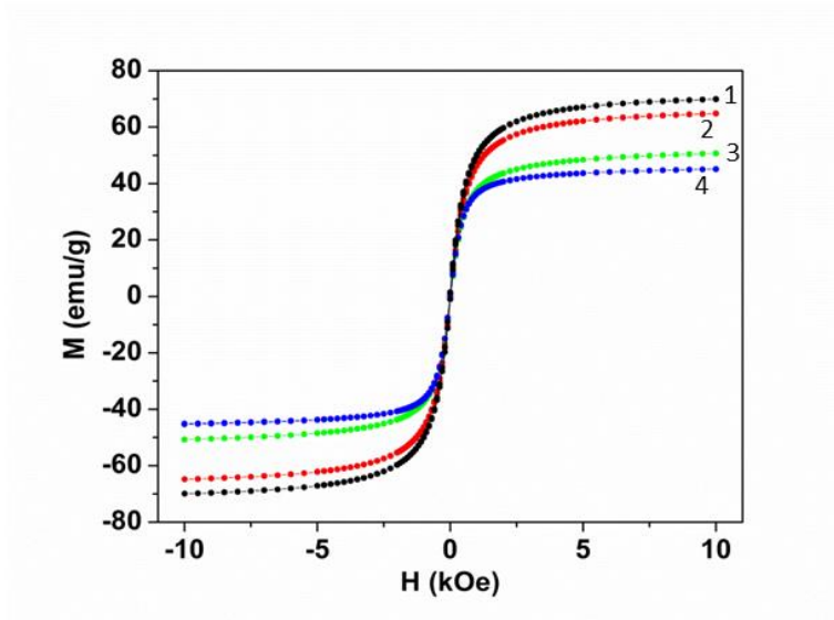
Figure 6.2 M vs H plots for 1. S1 (black), 2. S2 (red), 3. S3 (green) and 4. S4 (blue) nanoparticle samples at 300 K.
