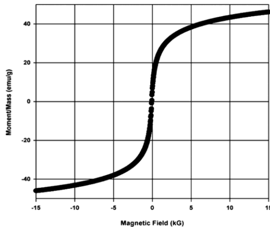
Figure 1.4 Magnetization ( M ) vs Magnetic Field ( H ) plot for \gamma - \text{Fe}_2\text{O}_3 nanoparticles showing superparamagnetic behavior [25].
