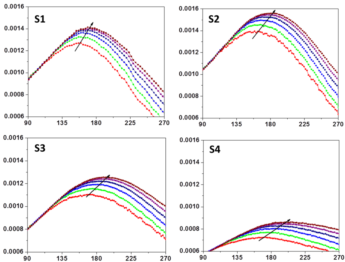
Figure 6.4 Out-of-phase susceptibility ( \chi'' ) vs Temperature (T) graph for S1, S2, S3 and S4 nanoparticle samples at six different frequencies of 500 Hz (red), 650 Hz (green), 800 Hz (blue), 950 Hz (navy), 1100 Hz (purple) and 1250 Hz (wine) under an excitation field of 10 Oe.
