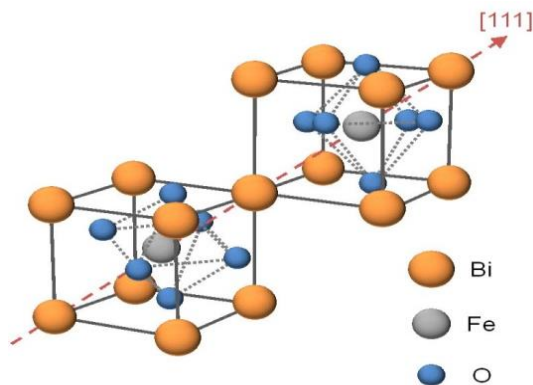
Figure 7.1 Perovskite structure of \text{BiFeO}_3 crystals [153]
