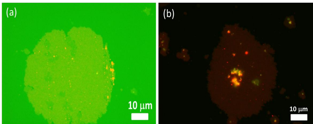
Figure 8.2 Images of SLBs after FITC addition and 30 minutes of incubation (a) after 10 washings with PBS (b) after 20 washings with PBS.
