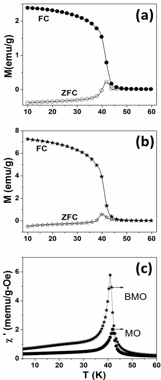
Figure 5.5 Zero-field-cooled (ZFC) and field-cooled (FC) magnetization curves for (a) MO and (b) BMO nanoparticles measured at 100 Oe. (c) In-phase susceptibility ( \chi' ) vs Temperature ( T ) graph for MO and BMO nanoparticles at a specific frequency of 10kHz under an excitation field of 10 Oe.
