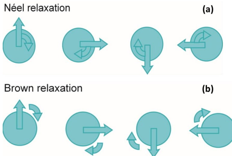
Figure 1.13 (a) The Néel relaxation shows the rotation only the magnetic spin with the particle being fixed (b) The Brownian relaxation indicates the physical rotation of the entire particle. (Image by courtesy of nanotherics.com)
