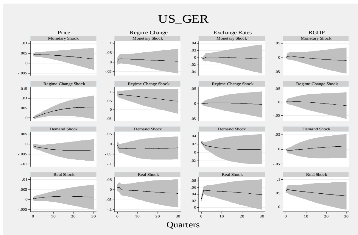
Figure 2: Impulse Responses (Regime Change)
