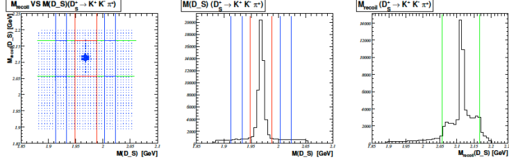
Figure 3.4: M_{recoil} vs. M_{D_s} distribution of channel D_s \rightarrow KK\pi from signal MC sample. Red and Green lines reflect signal cuts, blue line shows sideband region
