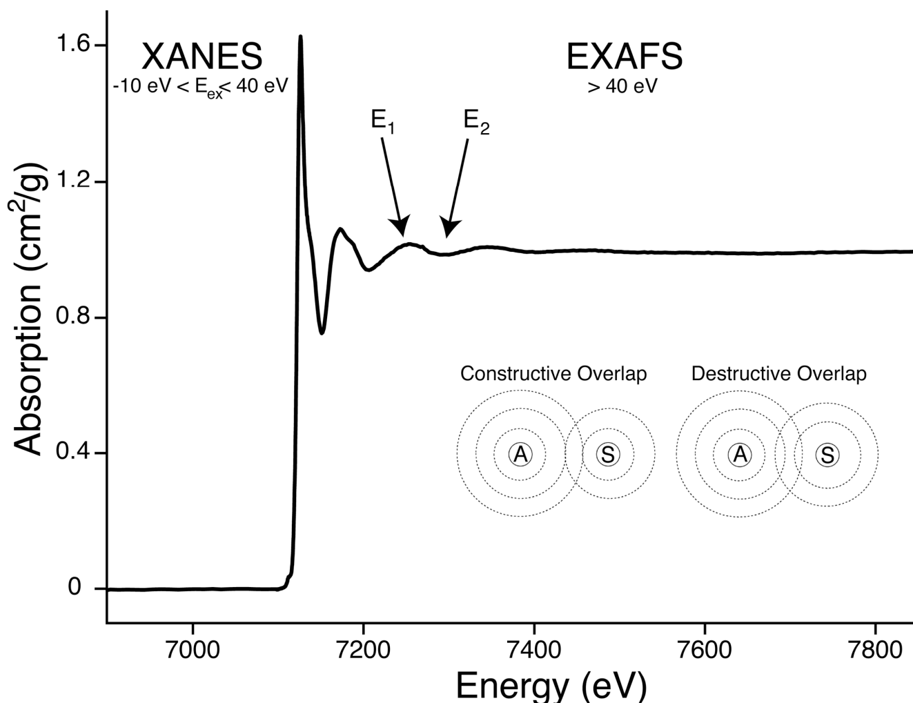
Figure 1: Iron K-edge XAS spectrum from ferrous ammonium sulphate. Spectra are divided into the XANES region ( \sim 10 eV to +40 eV relative to the large excitation signal) and the EXAFS region ( > 40 eV above the excitation edge). In the EXAFS region, absorption maxima ( E_1 ) and minima ( E_2 ) are highlighted. Inset: constructive and destructive overlap of photoelectron wave generated from excitation of the iron 1s core electron to the continuum.
